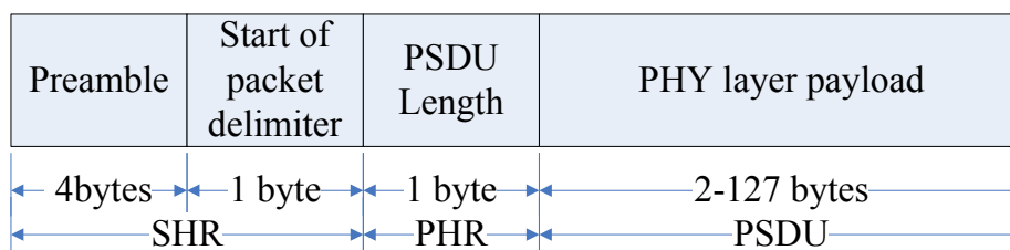
Fig. 8. IEEE 802.15.4 packet structure
