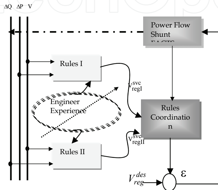
Fig. 8 Diagram of the proposed coordinated fuzzy approach
