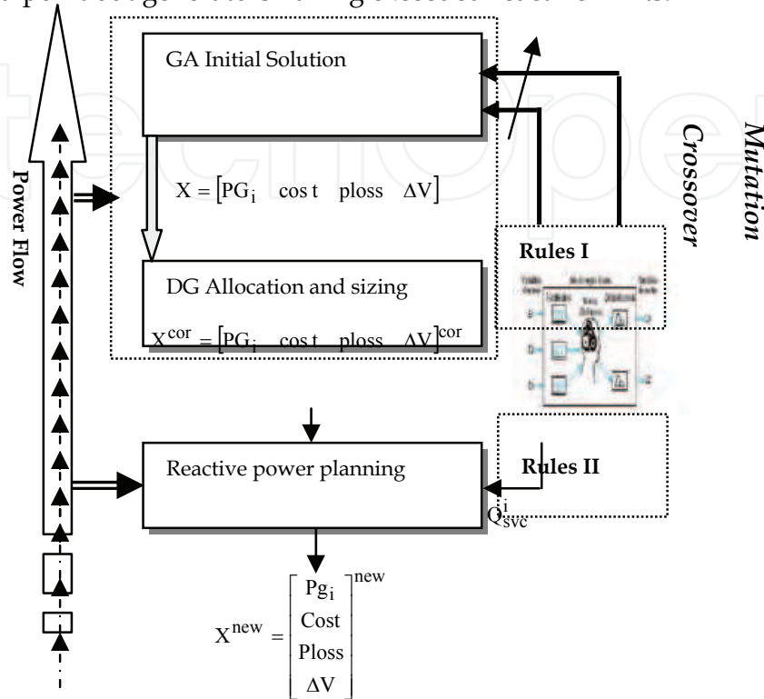
Fig. 3. Formulation mechanism of the proposed approach
