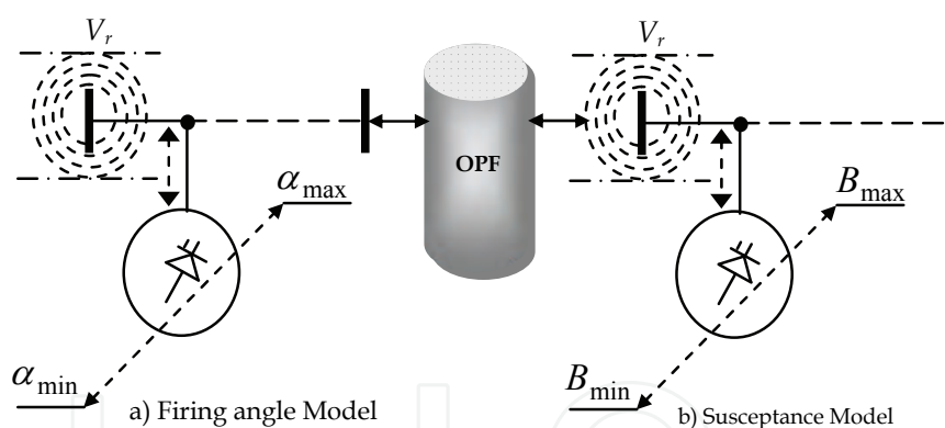
Fig. 12. Steady state model representation of SVC Compensator
