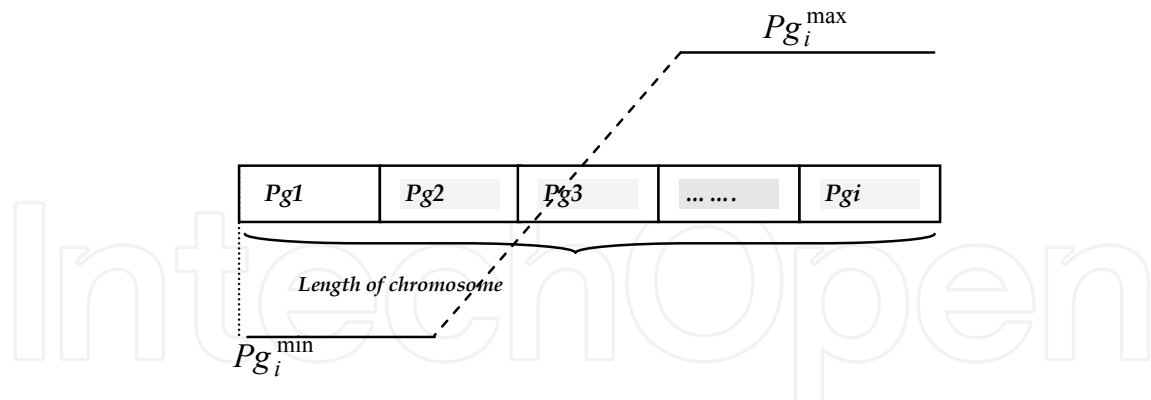
Fig. 5. Chromosome structure.
