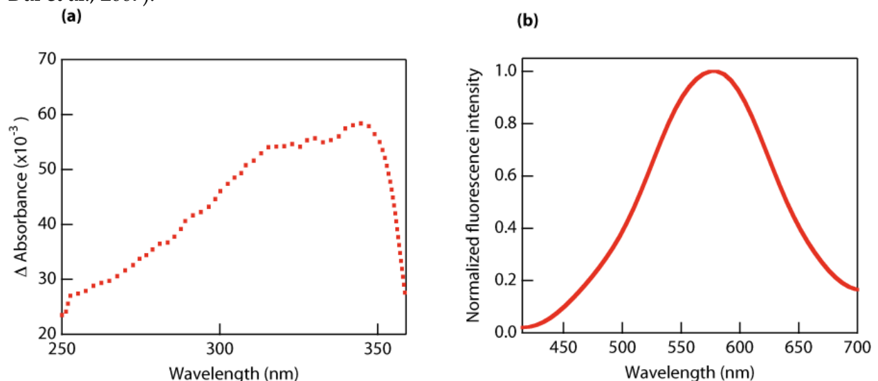
Fig. 1. (a) Differential absorbance spectrum between the irradiated and non-irradiated regions; (b) Emission spectrum (excitation wavelength, 405 nm) of the irradiated region. Experimental laser irradiation conditions: I = 6 \text{ TW}\cdot\text{cm}^{-2} , N = 10^6 . Differential absorbance and emission spectra are assigned to laser induced Ag clusters.
