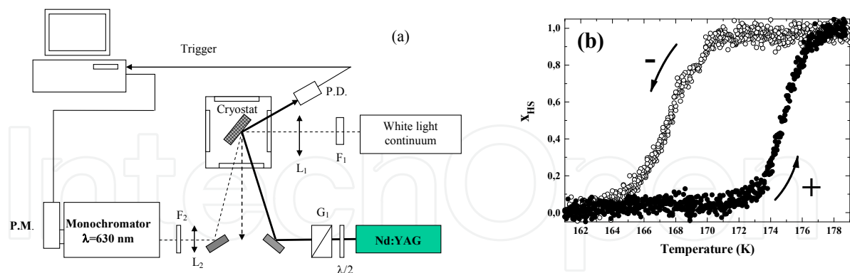
Fig. 6. (a) Sketch of the experimental set-up used to induce and measure the laser induced spin state transition. (b) Evolution of the reflected light versus the temperature. The temperature is either decreased from 180 K to 160 K or increased from 160 K To 180 K. X_{\text{HS}} is the molar fraction of molecules in the HS state.
