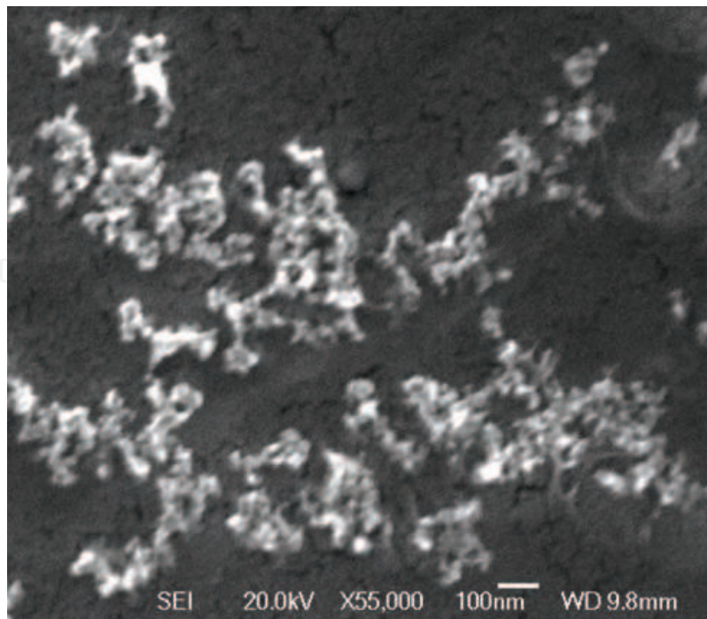
Fig. 5. High magnification SEM micrograph of \text{Al}_2\text{O}_3 nanoparticles
