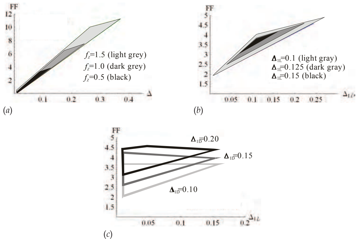
Fig. 8. (a) Region of correct DC behaviour FF vs \Delta = \Delta_1 = \Delta_2 for f_z = \{0.5, 1.0, 1.5\} . (b) FF vs. \Delta_{ID} = f_z - f_z for \Delta_{IL} = f_A - f_B = \{0.1, 0.125, 0.15\} and (c) FF vs. \Delta_{IL} for \Delta_{ID} = \{0.1, 0.15, 0.20\} , with \Delta_2 = 0.1 .
