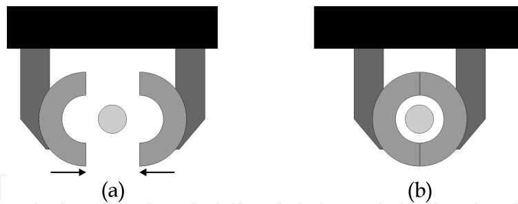
Fig. 8. The power pick-up device with the clasp mechanism. (a) Opened power pick-up device. (b) Closed power pick-up device.
