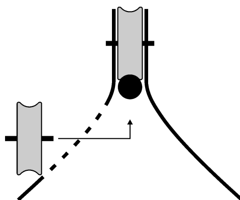
Fig. 5. A part of the proposed drive mechanism. After the robot lands on the conductor the lower wheels grasp the conductor from the sides.
