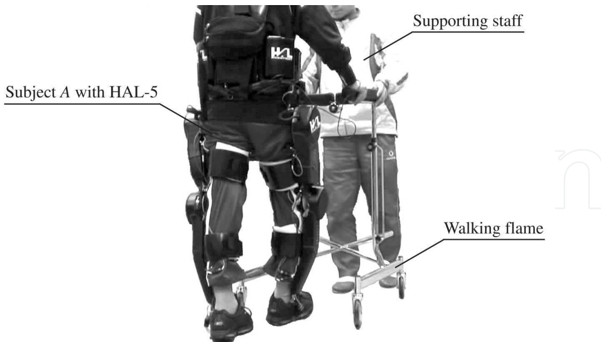
Fig. 9. Experimental setting.
