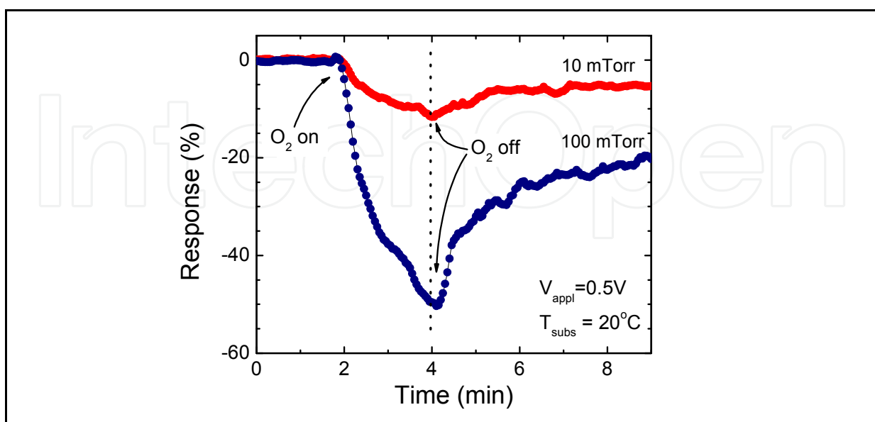
Fig. 13. Response to O_2 , suspended MWCNTs, O_2 peak pressures of 10 mTorr and 100 mTorr, respectively.
