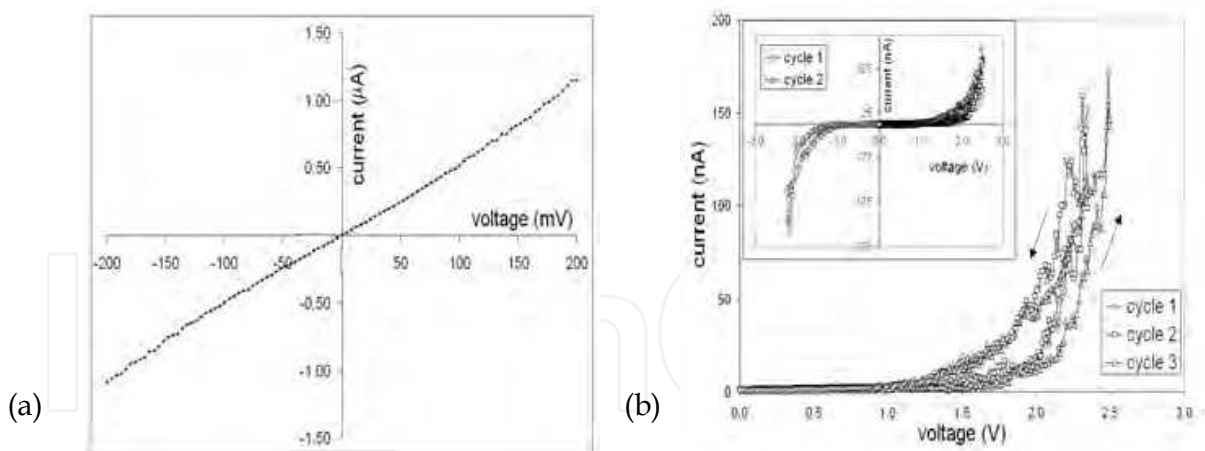
Fig. 4. a) Conduction measurements from the left Au/Ti electrode to the right electrode for a typical device gives R \sim 200 \text{ k}\Omega (trench width \sim 250 \text{ nm} , 2 \mu\text{m} \times 5 \mu\text{m} catalyst area). b) I-V characteristic of a device actuated over multiple cycles (250 nm trench width). The inset shows the ON state voltage to be similar in the forward-bias (pull electrode grounded) and reverse-bias (pull electrode positive) regimes, indicating that field emission is an unlikely possibility at these voltages (Kaul et al. , 2006).
