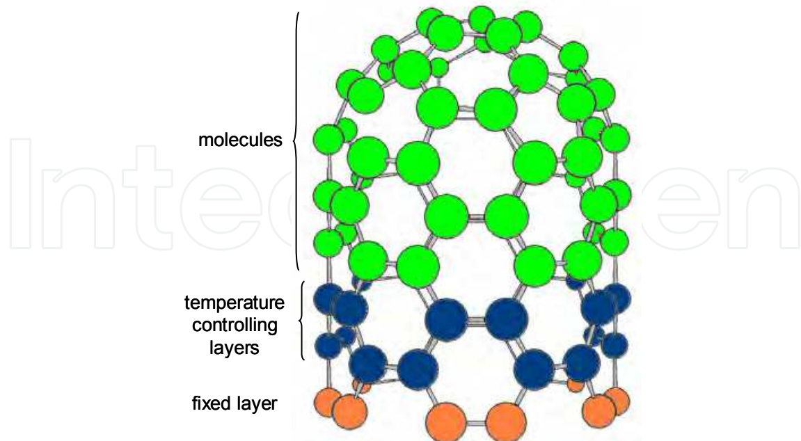
Fig. 2. Surface consisting of a capped carbon nanotube. The calculated system consists of 6 \times 6 units (2880 atoms) and has dimensions of 60 \text{ \AA} \times 52 \text{ \AA} \times 60 \text{ \AA} .
