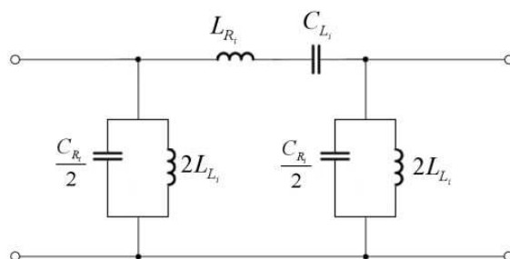
Fig. 2-2. Pi-equivalent circuit of the unit cell from the CRLH-TL
