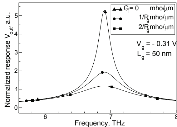
Fig. 3. Normalized HEMT frequency response at different leakage conductance G_l , L_g = 50 nm and V_g = -0.31 V.
