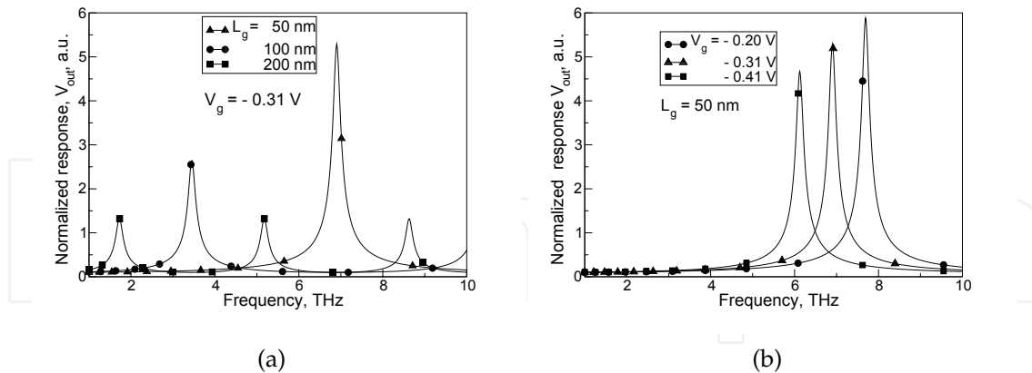
Fig. 2. Normalized frequency response of the HEMT at (a) different gate lengths and V_g = -0.31 V; and (b) different gate bias voltages and L_g = 50 nm.
