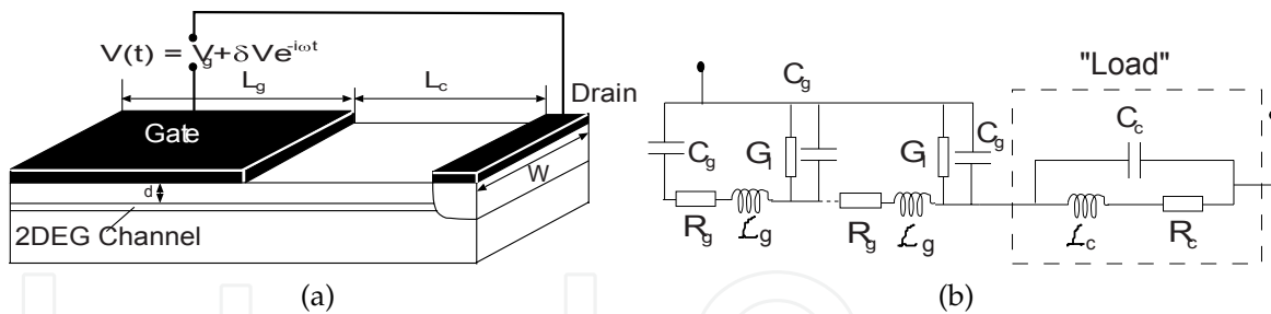
Fig. 1. Schematic structure of the HEMT (a) and its electric equivalent circuit (b). Gated portion of the 2DEG channel is represented by distributed R\mathcal{L}C circuit. The rest part of the device including ungated and contact regions is enclosed in a dashed box and treated as a "load".
