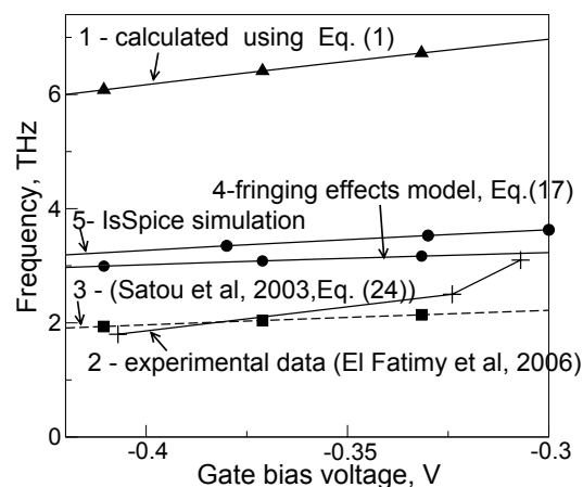
Fig. 9. Fundamental frequency of plasma oscillations: 1– Ideal case, calculated using Eq. (1); 2 – Experimental data extracted from Ref. (El Fatimy, 2006); 3 – Model for impact of ungated regions, Eq. (24) of Ref. (Satou,2003); 4 – model accounting for fringing effects, Eq. (17); 5 – Results of IsSpice simulation.
