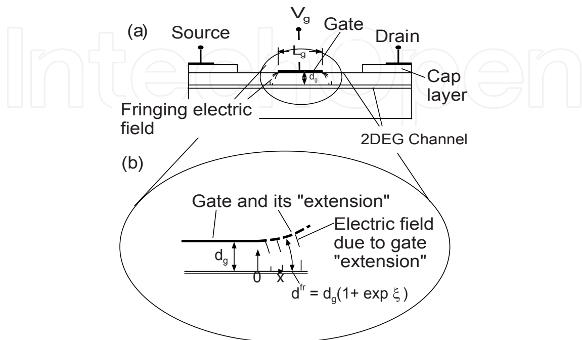
Fig. 5. Schematic of the HEMT structure (a) and model of "extended" gate (b).
