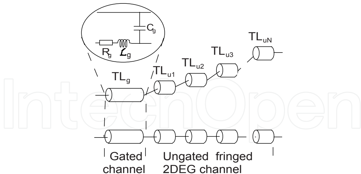
Fig. 7. Cascaded TL model for the HEMT in the presence of fringing effects. Gated 2DEG channel is represented by a single uniform TL. Ungated fringed 2DEG channel region is partitioned so that each part can be represented by uniform TL ( TL_{u1} , TL_{u2} ,... TL_{uN} ).
