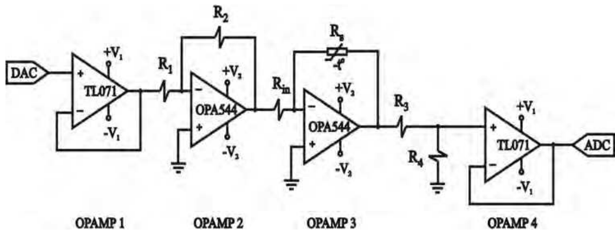
Fig. 2. Developed electronic circuit schematics
