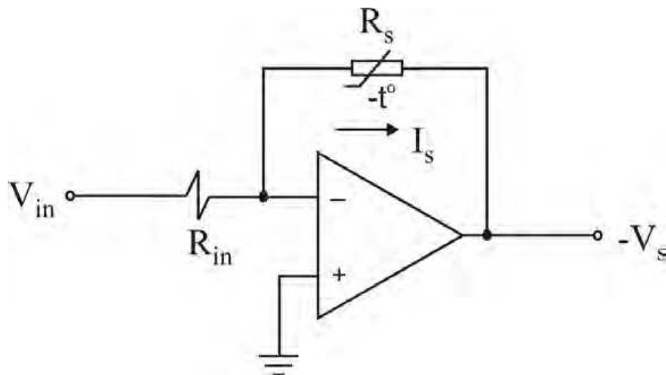
Fig. 3. Electronic sub-circuit.
