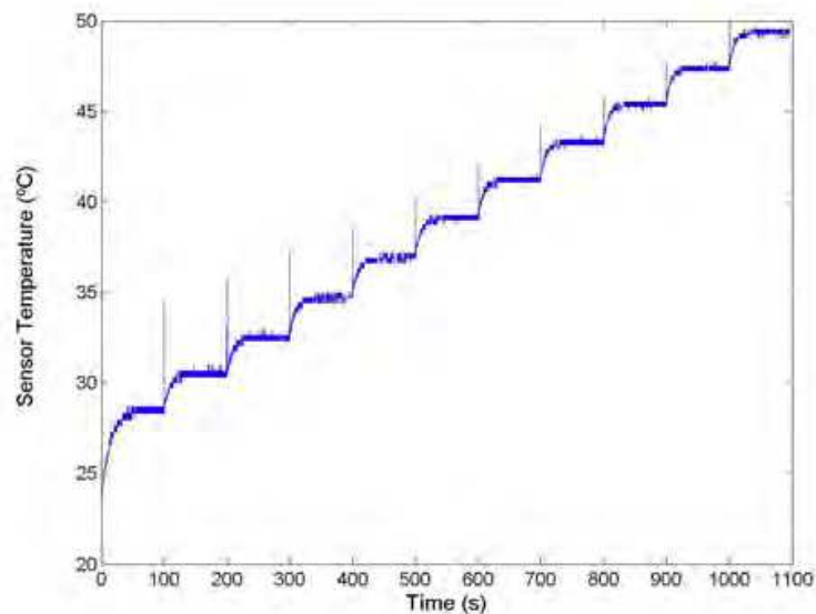
Fig. 5. Output temperature with input in increasing steps (non-linearized system).
