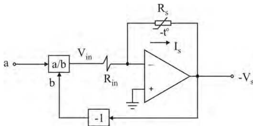
Fig. 4. Electronic sub-circuit with feedback linearization.
