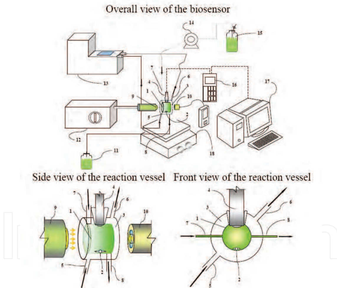
Fig. 1. Schematic diagram of the photosynthetic activity measurement system. 1 reaction cell, 2 magnetic bar, 3 cooling water jacket, 4 dissolved oxygen electrode, 5 inlet of cooling water, 6 outlet of cooling water, 7 inlet of sample, 8 outlet of sample, 9 convex lens, 10 quantum sensor, 11 wastewater, 12 quartz halogen illuminator, 13 water bath, 14 peristaltic pump, 15 sample reservoir, 16 dissolved oxygen meter, 17 computer and 18 magnetic stirrer.
