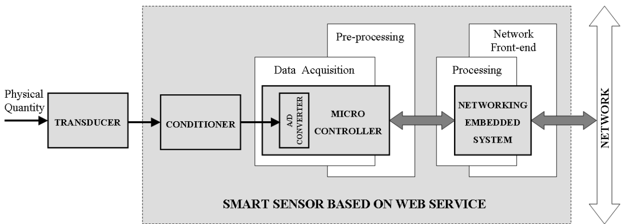
Fig. 4. Simplified block diagram of a Smart Sensor
