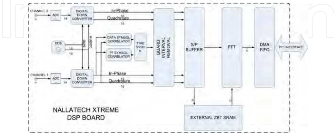
Fig. 14. Architecture of SDR receiver
