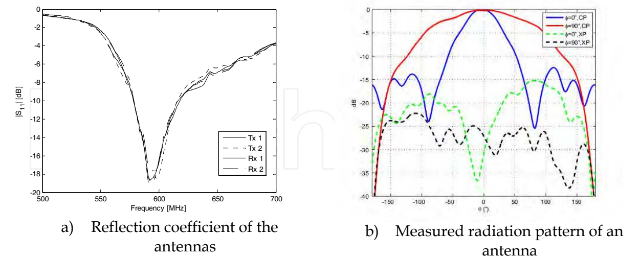
Fig. 18. Antenna performances
