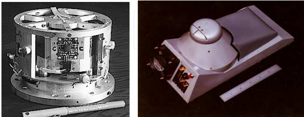
Fig. 2. (a) UBC Teleoperation Master, (b) UBC Powermouse
