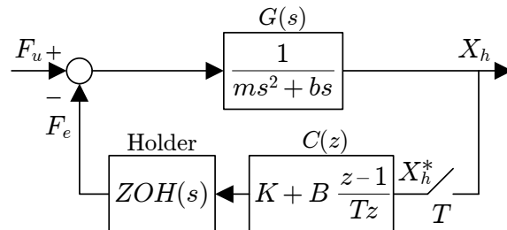
Fig. 2. Discrete haptic model.
