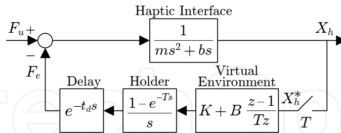
Fig. 4. Linear simplified model of a haptic system.
