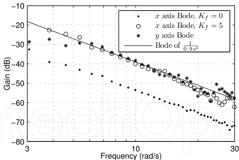
Fig. 25. Experimental gain Bode diagrams of the LHIfAM along y axis (stars), and along x axis with K_f = 0 (dots) and K_f = 5 (circles).
