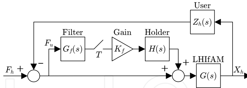
Fig. 22. Sampled model of the system in free movement.
