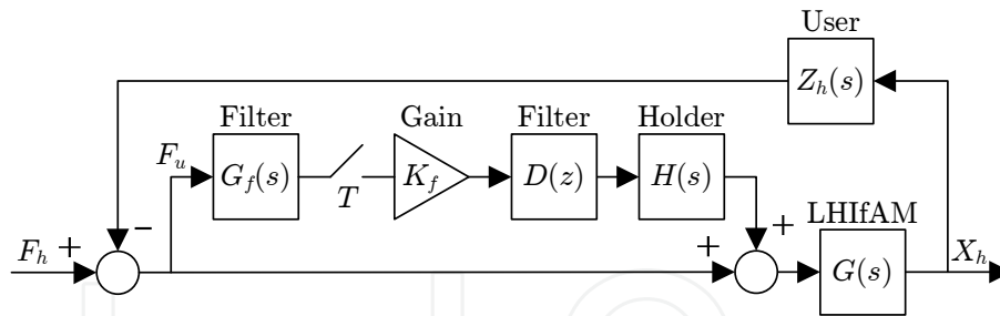
Fig. 24. Final force feedforward strategy with digital filter.
