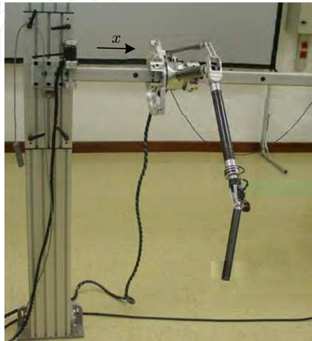
Fig. 7. LHifAM haptic interface.
