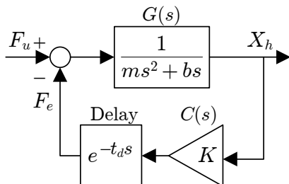
Fig. 1. Continuous haptic model.
