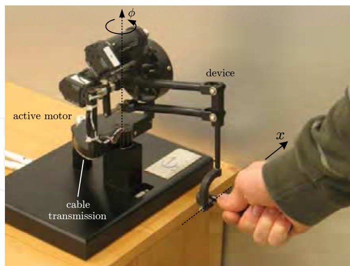
Fig. 13. PHANToM 1.0 haptic interface.
