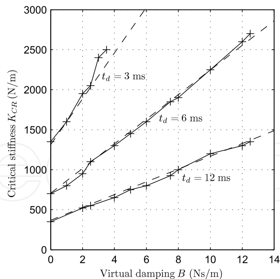
Fig. 10. Experimental stability boundaries for the LHfAM and a delay t_d of 3, 6 and 12 ms (pluses and solid) and theoretical stability boundaries for a physical damping b of 4.6 Ns/m (dashed) and same delays.
