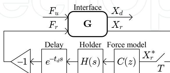
Fig. 12. Haptic system with impedance interaction.
