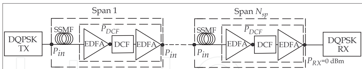
Fig. 11. Scheme of the DQPSK transmission system.
