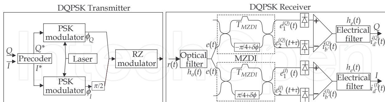
Fig. 1. Scheme of the DQPSK transmitter and receiver.
