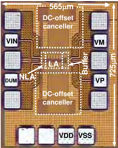
Fig. 34. Micrograph of the pulse receiver.
