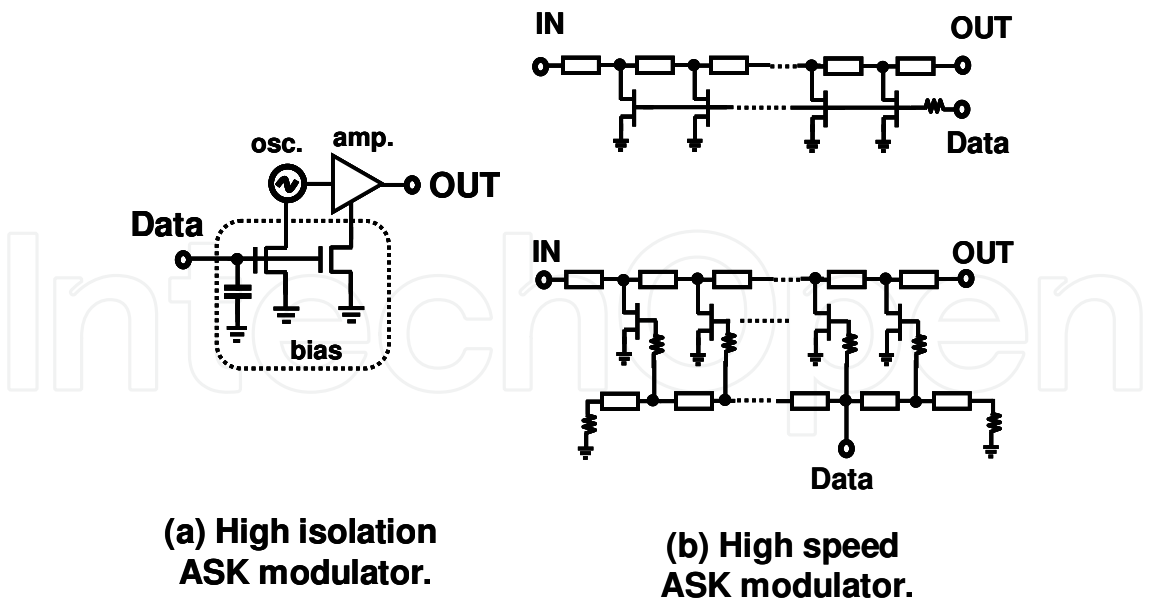
Fig. 10. Architectures of conventional (a) high-isolation and (b) high-speed ASK modulators.
