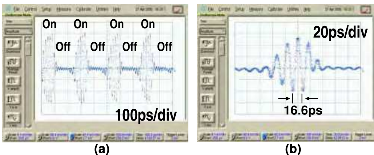
Fig. 19. Measured output response of the modulator for (a) an 8Gbps data train and (b) a single 125ps data pulse.
