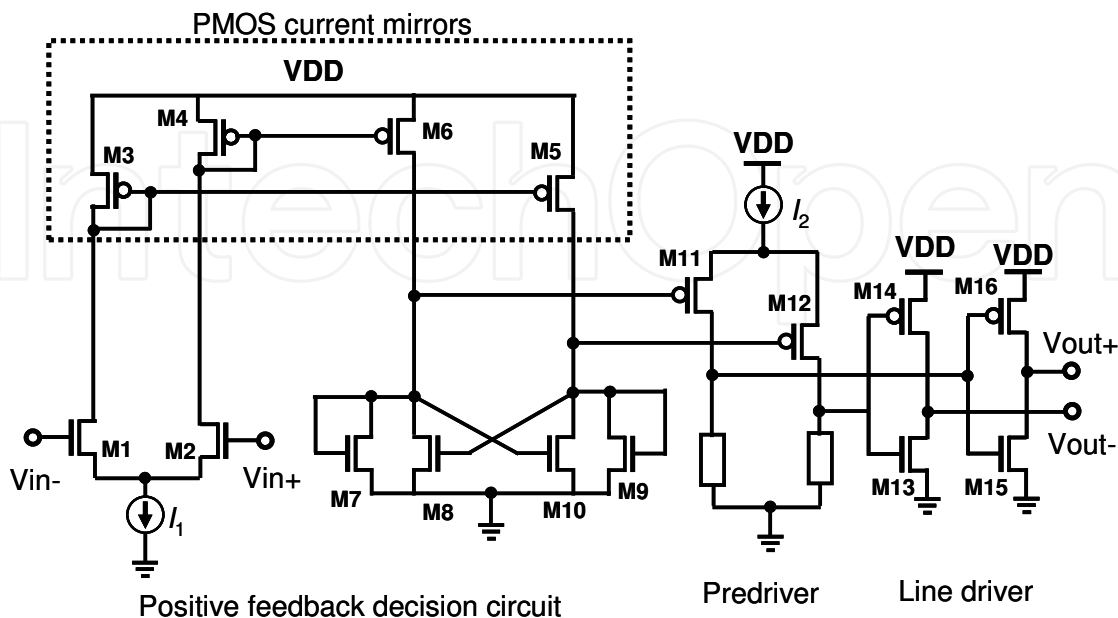
Fig. 42. High-speed CMOS comparator with hysteresis.
