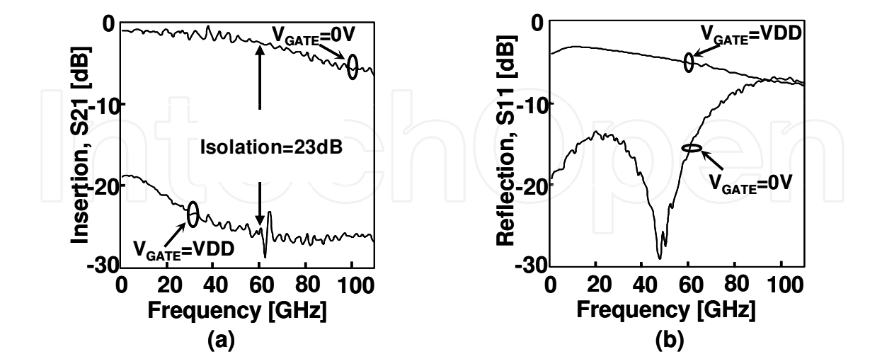
Fig. 28. Measured (a) insertion loss (S21) and (b) reflection loss (S11) of the ASK modulator for ON and OFF states.
