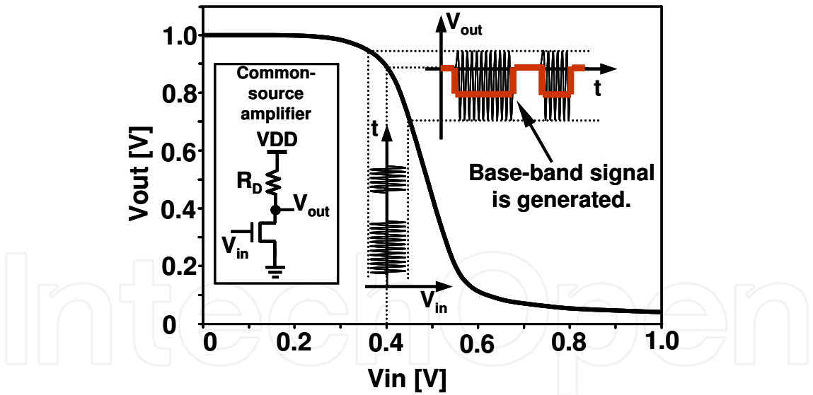
Fig. 33. Nonlinear pulse detection using a common-source amplifier.
