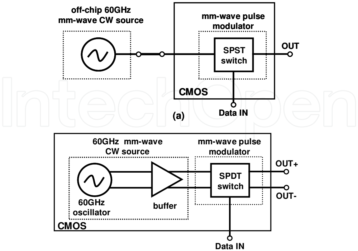
Fig. 22. Architecture of (a) a single-ended millimeter-wave pulse transmitter with off-chip 60GHz CW source and (b) a proposed differential-ended pulse transmitter with on-chip 60GHz CW source.
