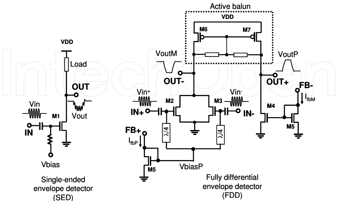
Fig. 40. Millimeter-wave CMOS envelope detector circuits.
