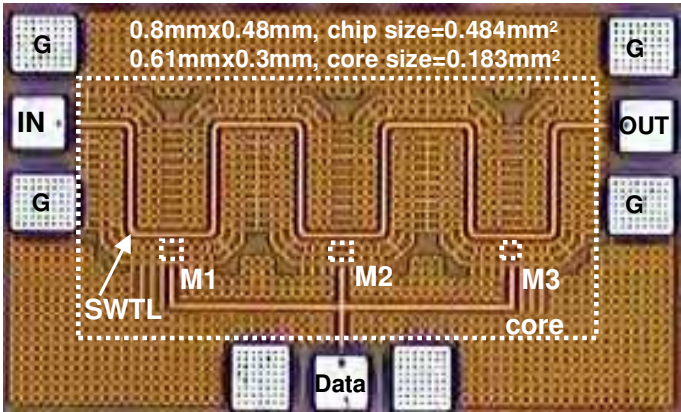
Fig. 17. Micrograph of the fabricated chip.
