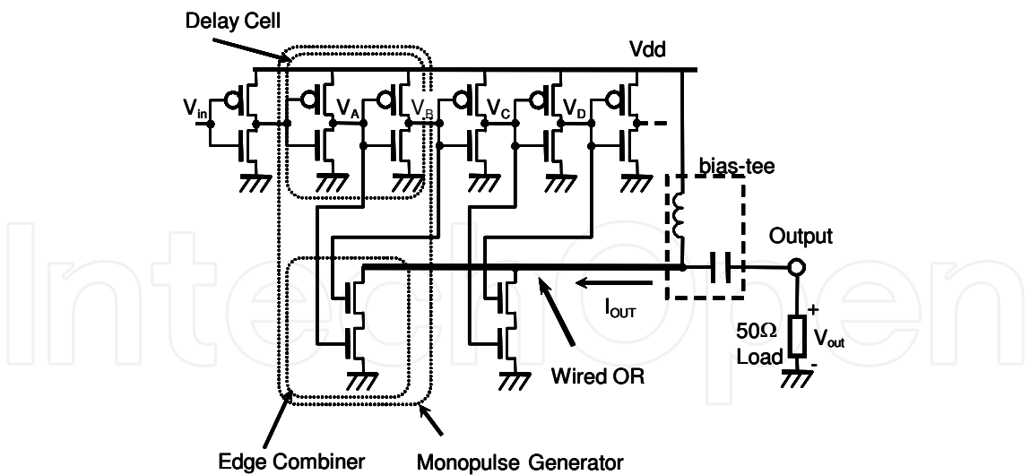
Fig. 2. Circuit topology of a 60GHz CMOS pulse generator.
