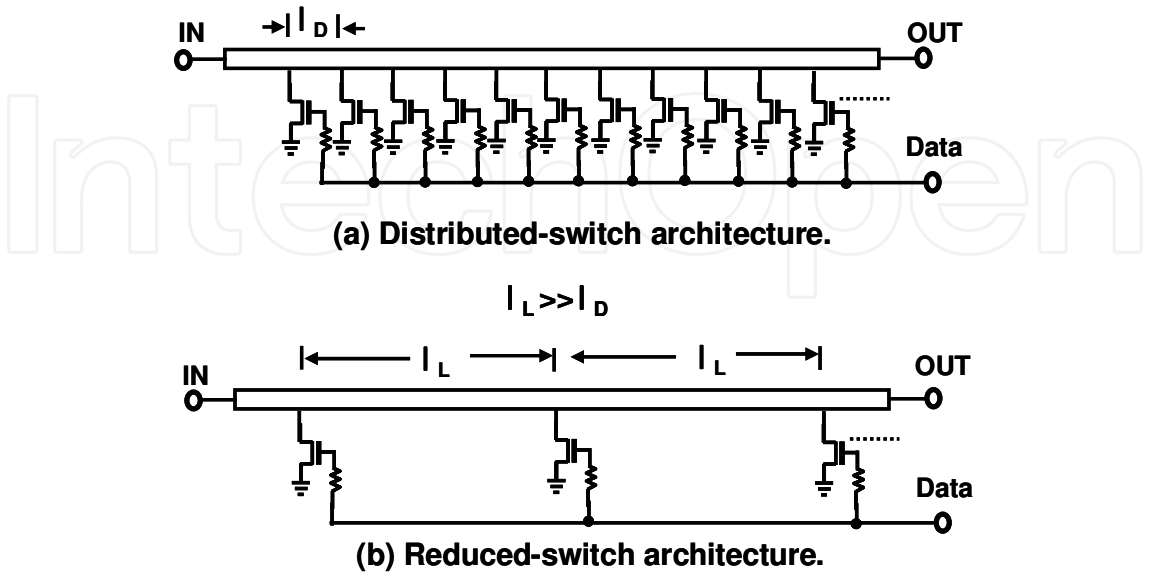
Fig. 11. Architectures of (a) distributive and (b) reduced-switch ASK modulators in CMOS process.
