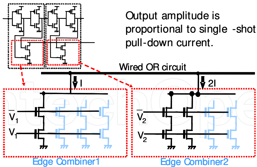
Fig. 5. MOSFET sizing for generating pseudo-raised cosine pulse.
