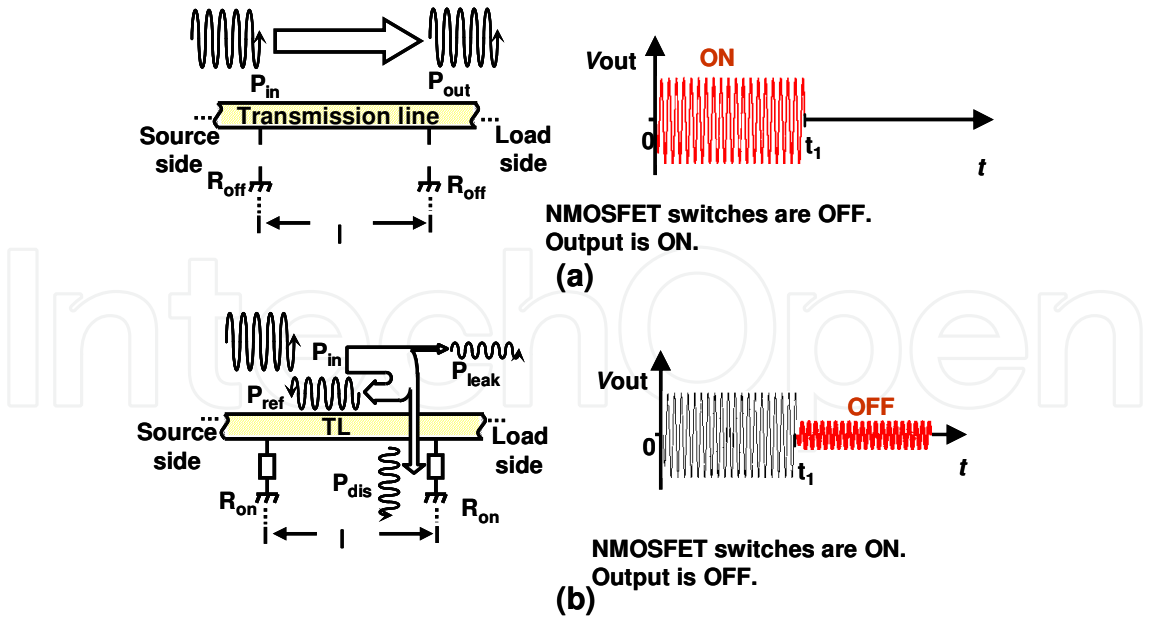
Fig. 12. Illustration of transmitted, reflected, dissipated and leaked signals of a switch in the (a) ON and (b) OFF states of the modulator when the millimeter-wave signal travels from source to the load.
