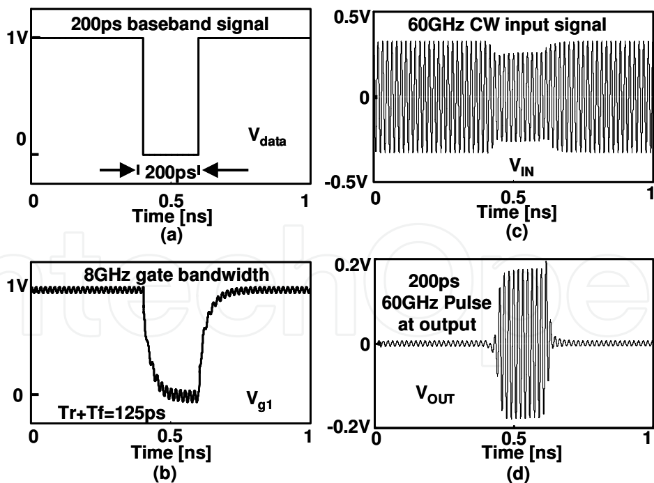
Fig. 16. Transient simulation; (a) 200ps applied data pulse, and responses of (b) the gate voltage of the NMOSFET switch, and (c) input and (d) output signals. voltages is estimated as 125ps, which corresponds to the maximum data rate of 8Gbps. The 60GHz millimeter-wave ASK modulator is fabricated by a 6-metal 1-poly 90nm CMOS
