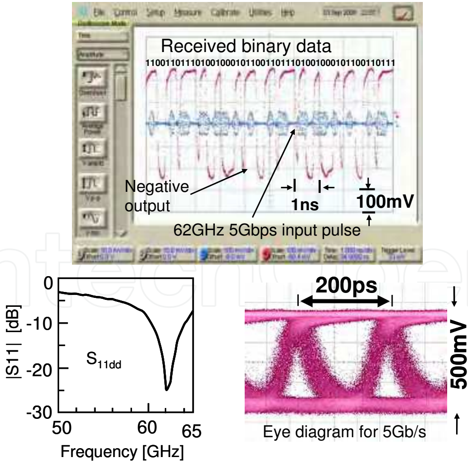
Fig. 44. Summary of measured results of the receiver.
