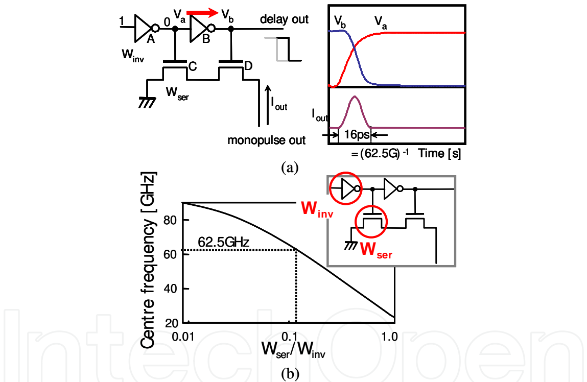
Fig. 3. (a) An edge combiner comprising MOSFETs C and D has to generate a 16ps pulse. (b) Centre frequency as a function of NMOS width W_{ser} over inverter width W_{inv} .
