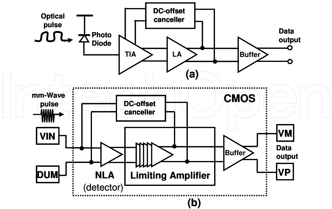
Fig. 32. (a) Typical optical receiver architecture and (b) diagram of receiver block in this work to realize the proposed pulse receiver.
