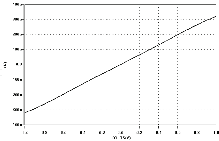
Fig. 9. V-I transfer characteristic
