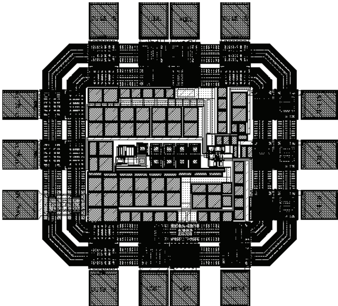
Fig. 16. The layout of proposed transconductor
