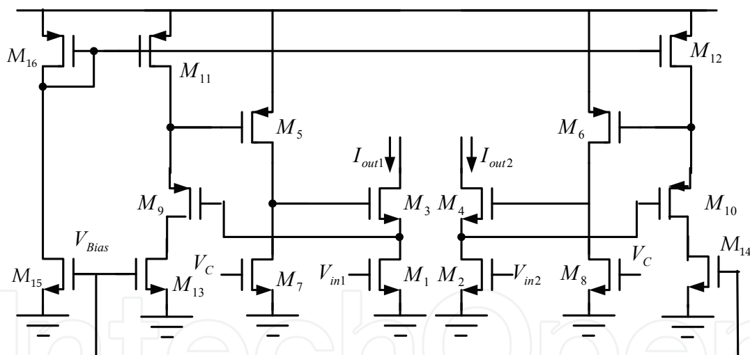
Fig. 8. The proposed transconductor
