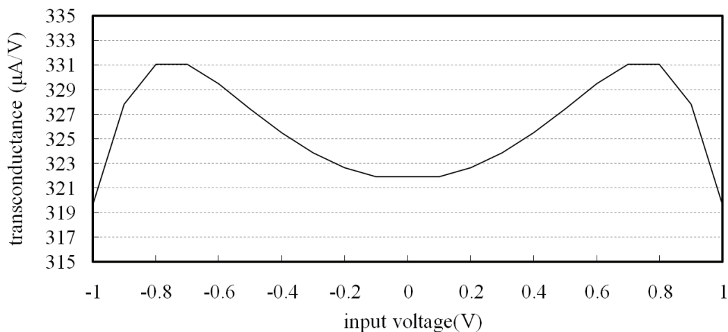
Fig. 10. The simulated transconductance at V_C=0.7V
