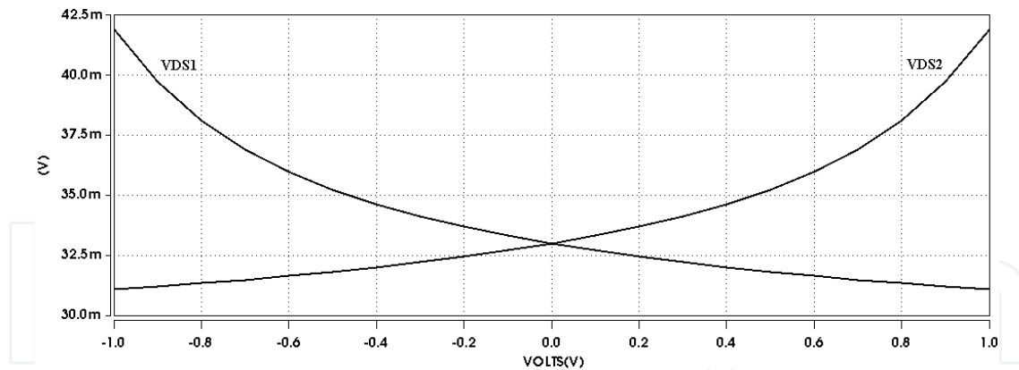
Fig. 11. The drain-source voltage of input transistor M_1 and M_2
