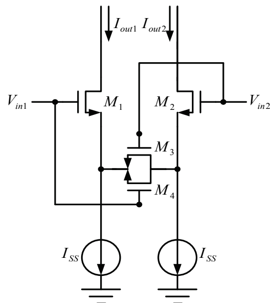
Fig. 5. Transconductor with source degeneration using MOS transistors
