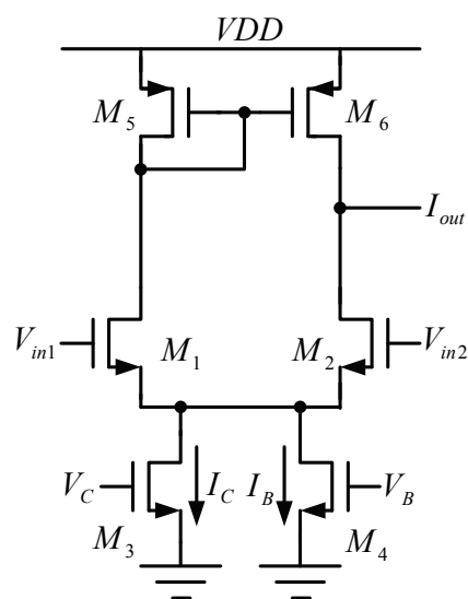
Fig. 6. Transconductor with adaptive biasing
