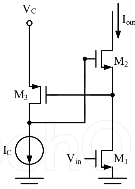
Fig. 3. RGC transconductor with PMOS gain stage
