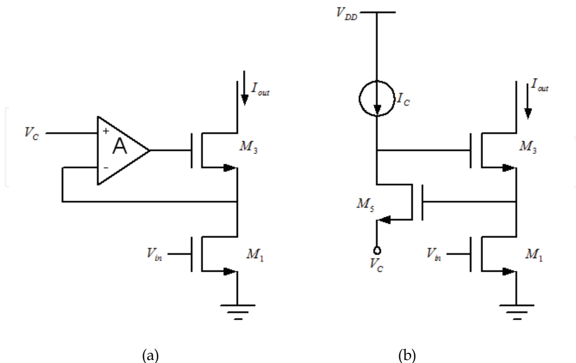
Fig. 2. (a) Basic triode transconductor structure (b) Simple RGC triode transconductor
