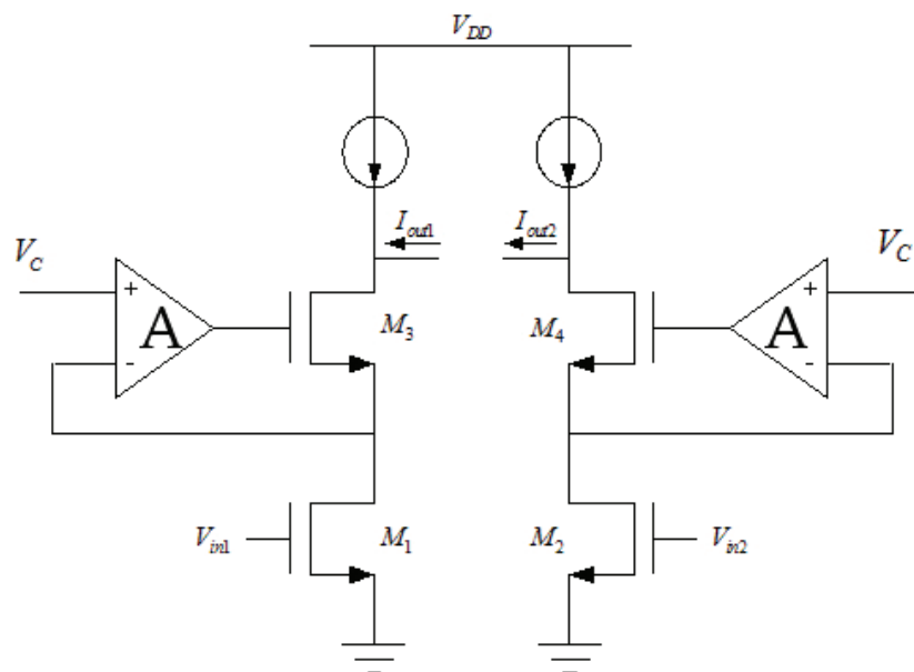
Fig. 1. Transconductor using constant drain-source voltage
