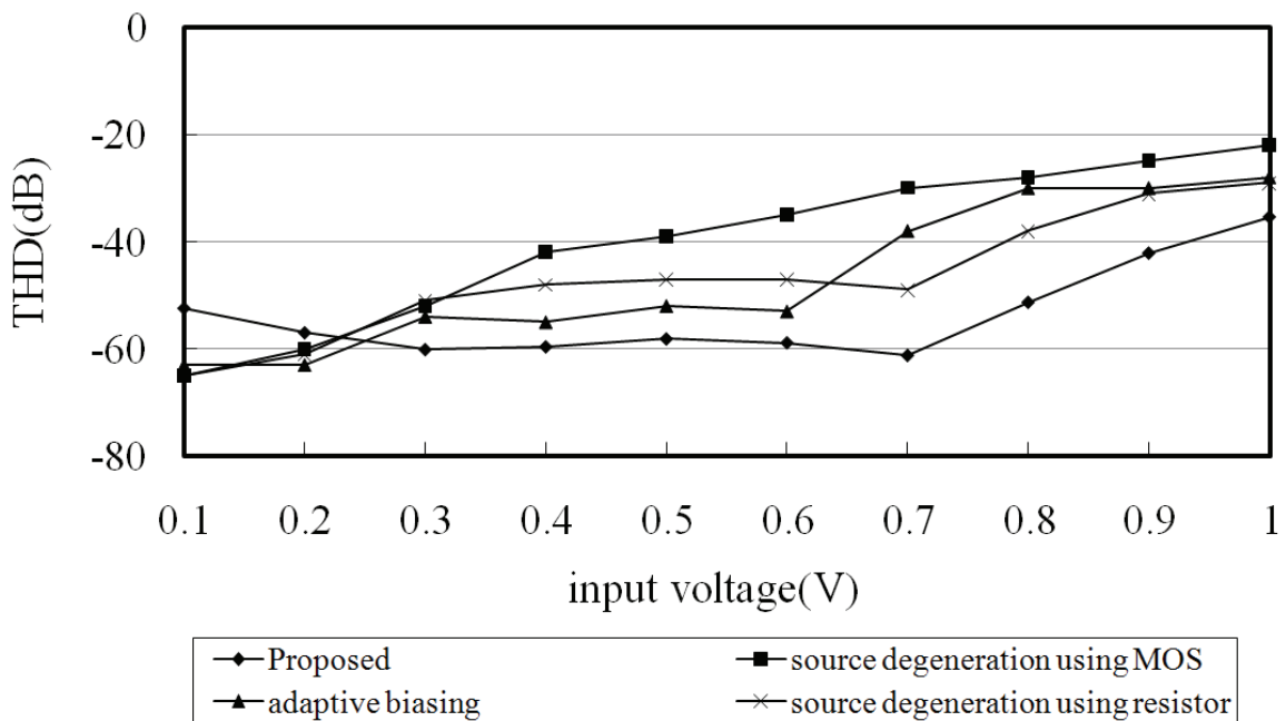
Fig. 15. Simulated THD at 1MHz for the four linearized transconductors
