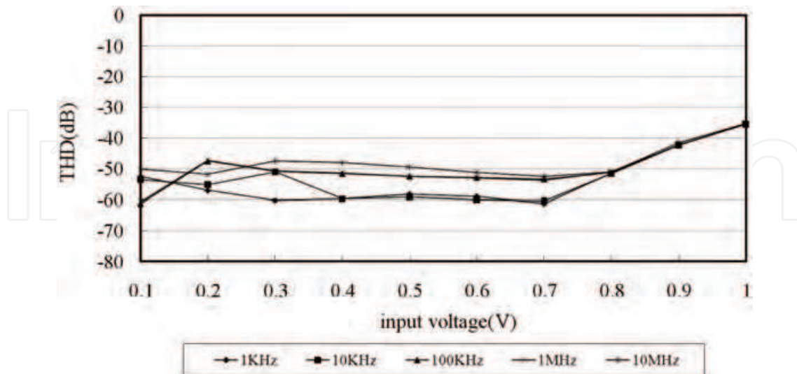
Fig. 12. Simulated THD for different input frequencies
