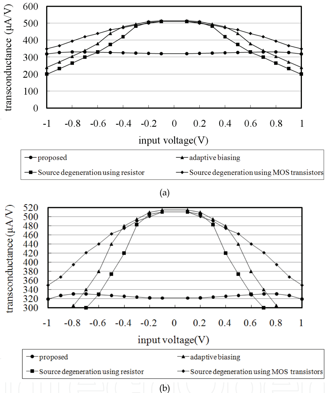
Fig. 14. Simulated transconductance for four linearization techniques (a) Full plot (b) Detail
