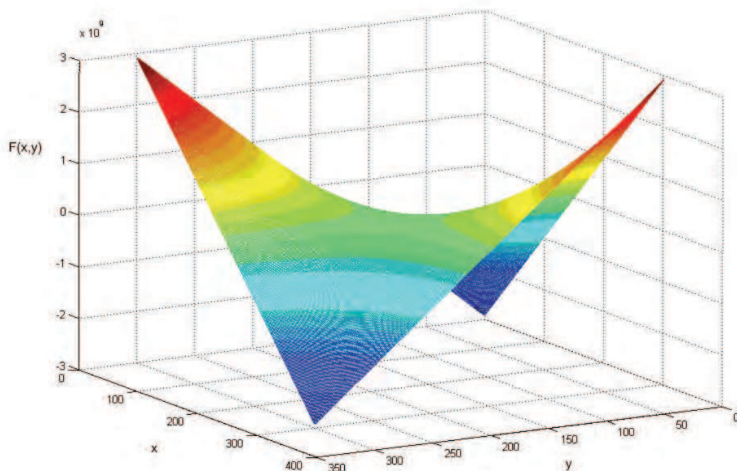
Fig. 2. Search space for the reduced Diophantine problem
