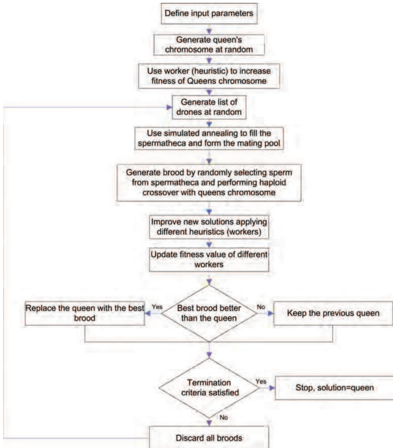
Fig. 1. Flowchart of HBMA algorithm
