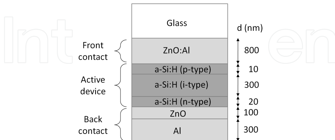
Fig. 5. Superstrate PVC configuration of single junction ( p-i-n ) structure
