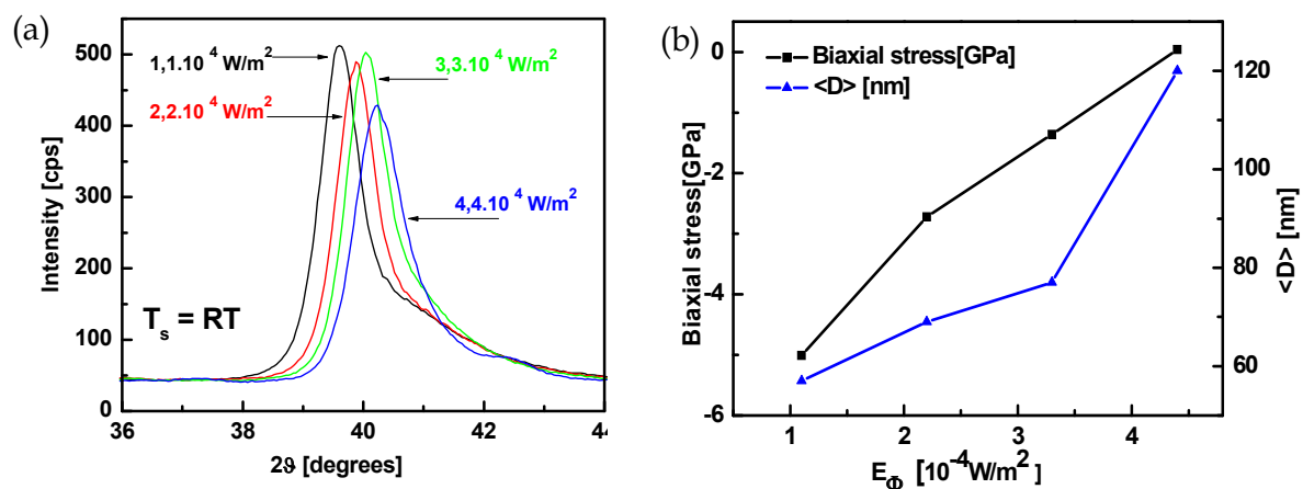
Fig. 13. AZO films sputtered at different power densities, E_\phi = 1,1 - 4,4 \cdot 10^4 \text{ W/m}^2 : (a) XRD patterns, (b) dependences of biaxial lattice stress and crystallite size on power density
