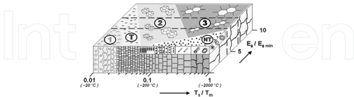
Fig. 1. Crystalline structure zone model of sputtered ZnO thin films: Zone 1 – porous structure of tapered amorphous or crystalline nanograins separated by voids, Zone T – dense polycrystalline structure of fibrous and nanocrystalline grains, Zone 2 – columnar grain structure, Zone 3 – single-crystal micrograin structure, Zone NT – nanostructures and nanoelements.
