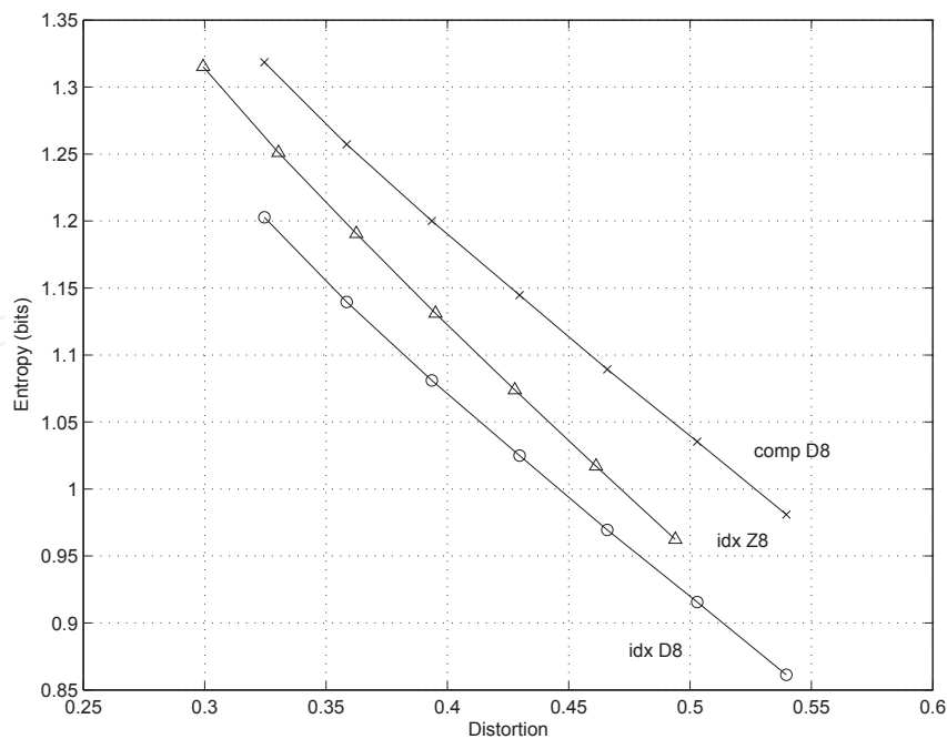
Fig. 3. Comparison of rate-distortion curves for Z_8 and D_8 lattice when the lattice vector components are entropy encoded (“comp”) and when the lattice vector indexes are entropy encoded (“idx”).
