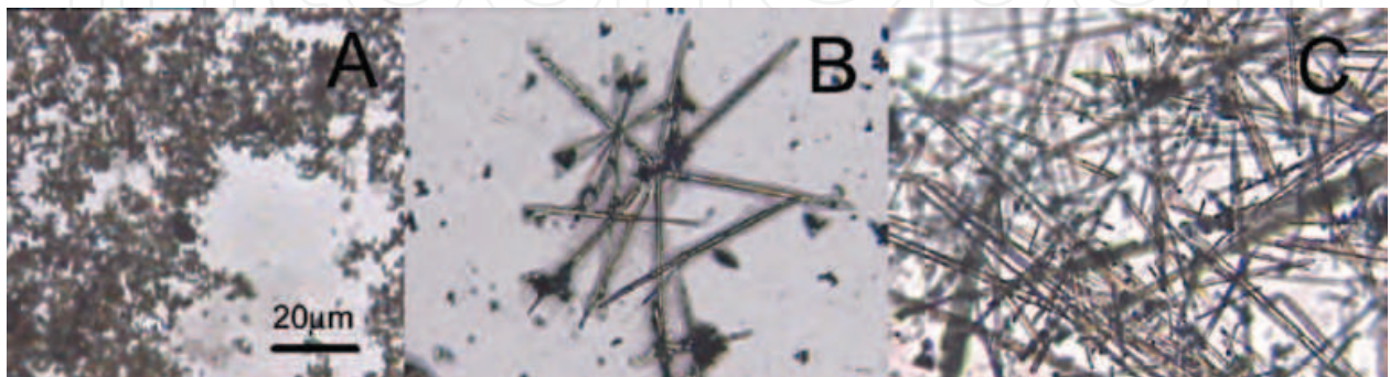
Fig. 4. Morphology of the hydrothermal products at 165 °C for different times of (A) 20, (B) 30, and (C) 40 h. Reproduced with permission from [60], X. Ding et al., Hyperbranched Polymer-Assisted Hydrothermal In situ Synthesis of Submicrometer Silver Tubes. Crystal Growth & Design 8, 2982 (2008).
