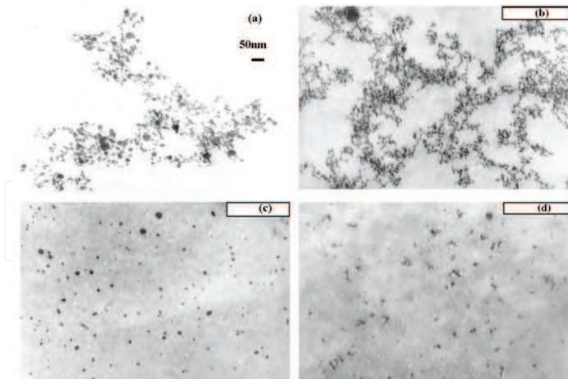
Fig. 2. TEM of AgNPs prepared with various NaBH 4 to AgNO 3 molar ratios at (a) 1/2, (b) 2, (c) 5, and (d) 10. Reproduced with permission from [57].
