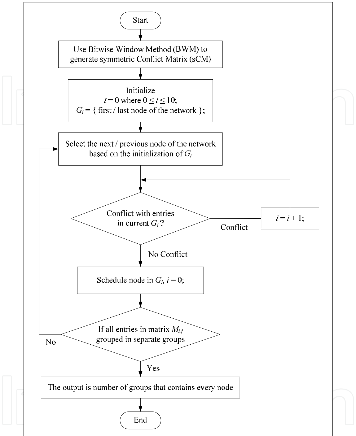
Fig. 7. General FastZ Algorithm Flowchart
