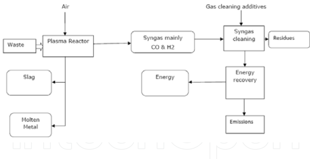
Fig. 12. Plasma gasification (Juniper 2006)
