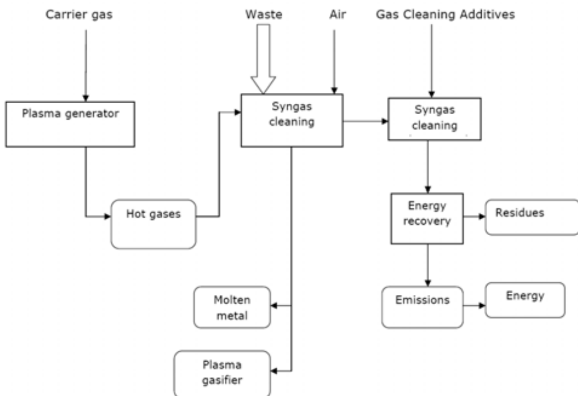
Fig. 11. “Plasma Assisted” gasification (Juniper 2006)
