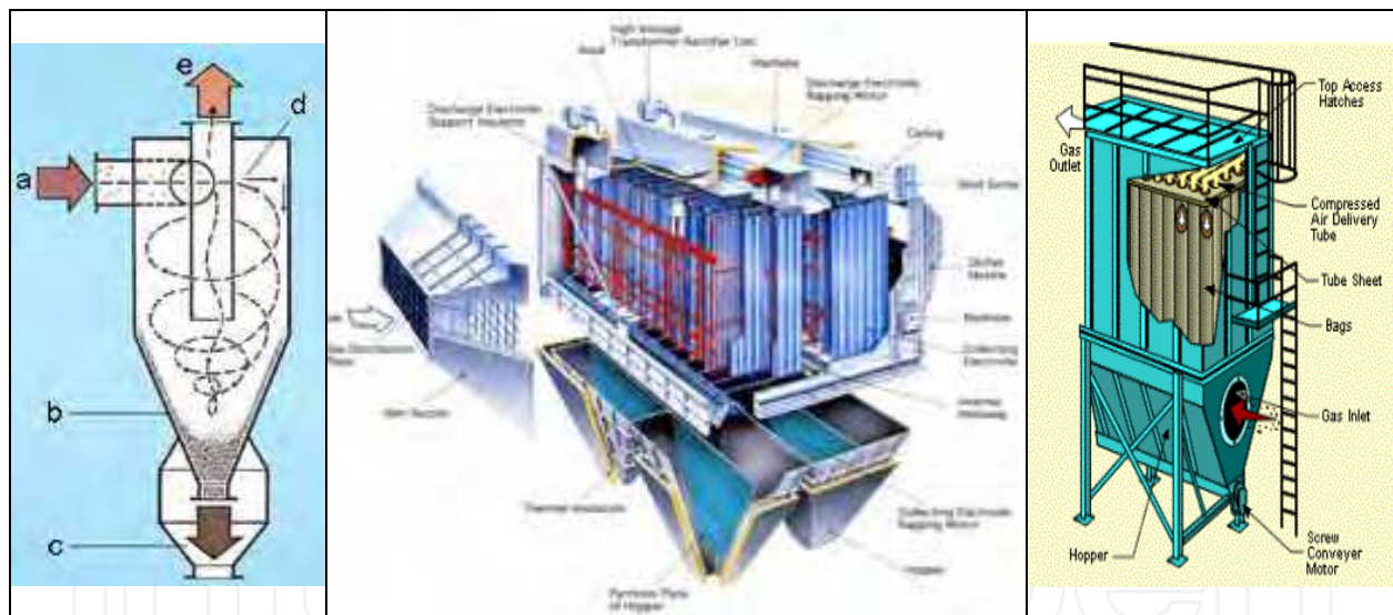
Fig. 5. Cyclones (left), electrostatic precipitators (middle) & bagfilters (right)
