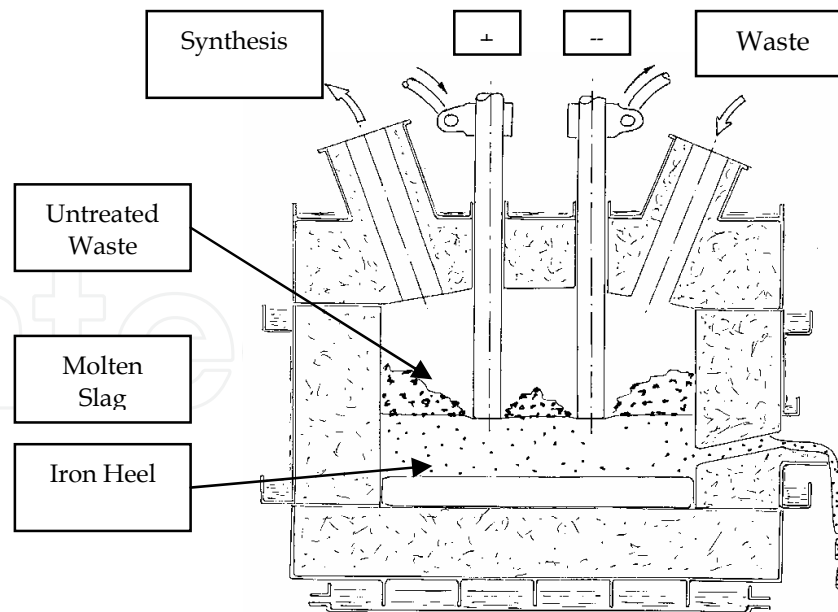
Fig. 13. Plasma Gasification / Vitrification Process
