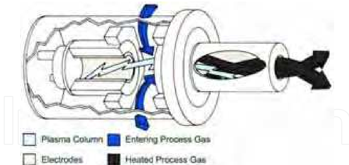
Fig. 9. Illustration of the operation of a plasma torch (Westinghouse)
