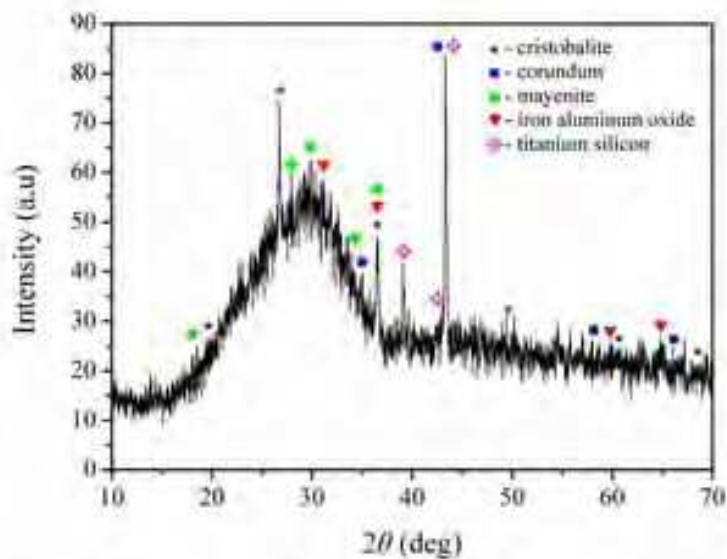
Fig. 18. XRD of the water quenched slag
