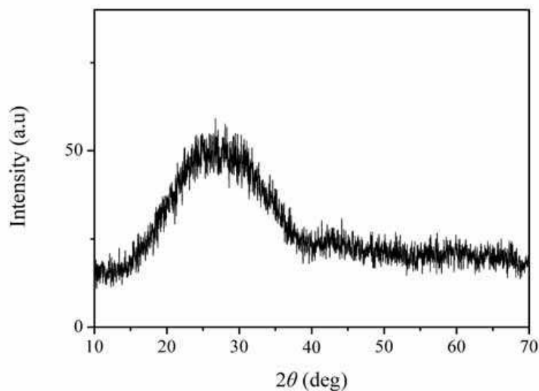
Fig. 19. XRD of the air-cooled slag
