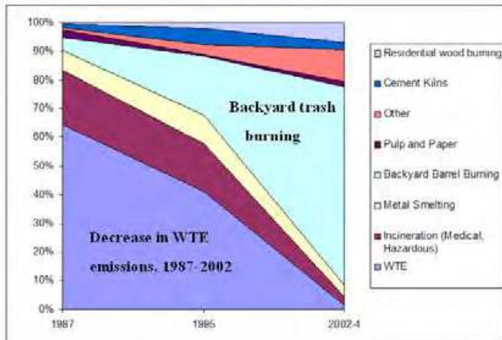
Fig. 4. Dioxins emission in the USA (Deriziotis, 2004).
