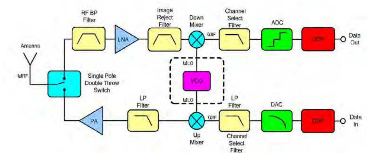
Fig. 1. Building blocks of super-heterodyne transceiver [2]
