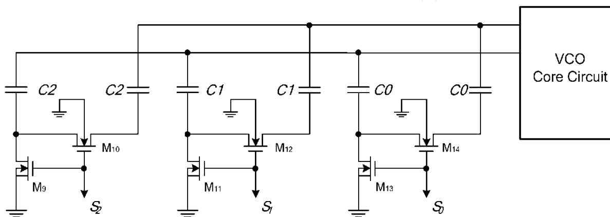
Fig. 11. A switching capacitor module
