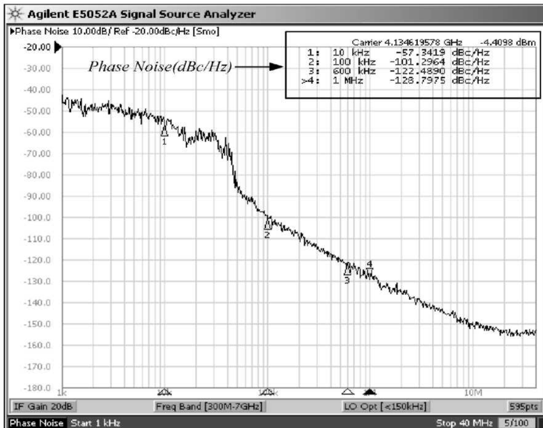
Fig. 15. Phase noise when S_2S_1S_0 = "100" , tuning voltage = 0V
