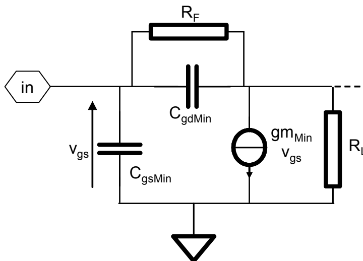
Fig. 6. Simplified model of a resistive feedback input stage
