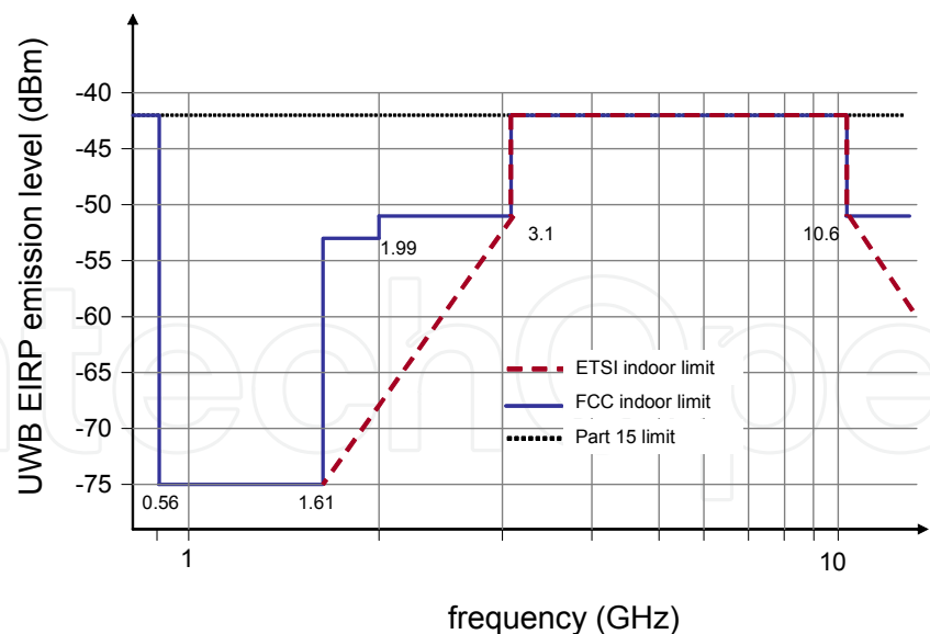
Fig. 1. UWB spectral mask for indoor communication systems [1]
