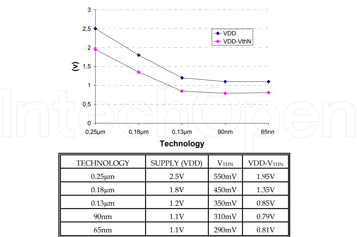
Fig. 5. CMOS scaling impact on VDD and V th
