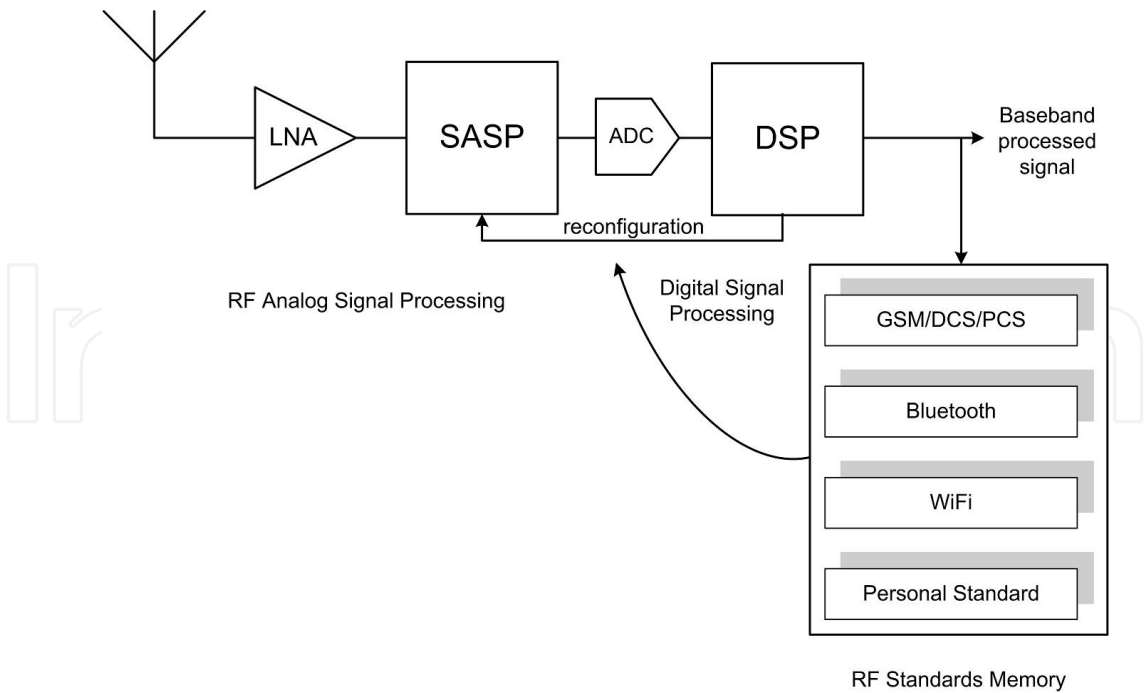
Fig. 32. A software defined radio solution [23]
