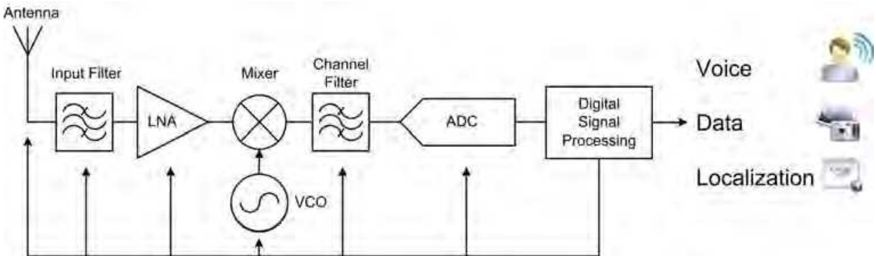
Fig. 31. A software defined radio solution based on conventional radio scheme
