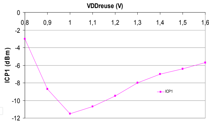
Fig. 24. ICP1 versus supply voltage
