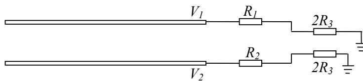
Fig. 4. Equivalent network for T-network termination in even-mode.
