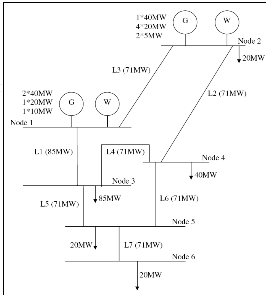
Fig. 7. Implemented version of the RBTS
