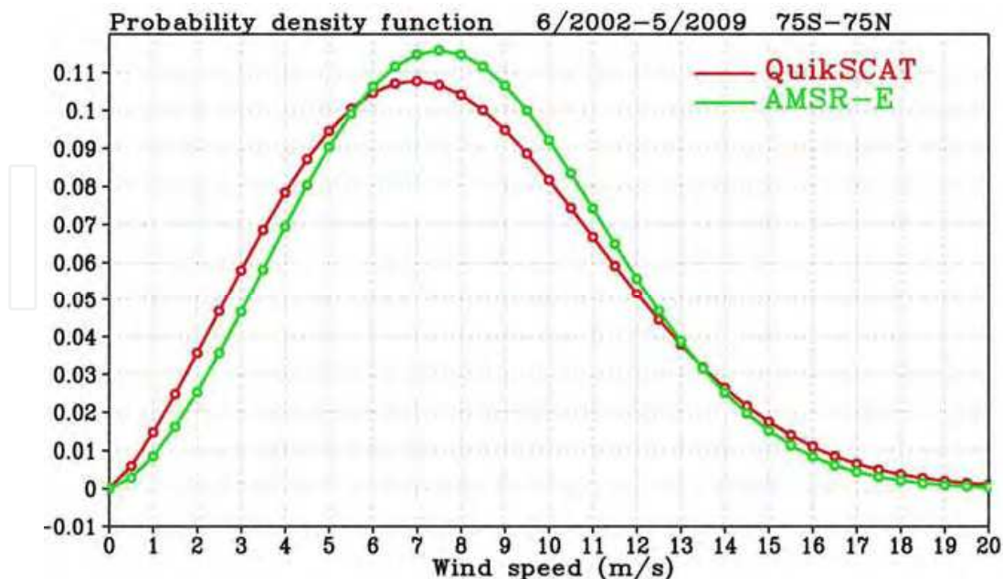
Fig. 1. Comparison of the probability density function of ocean surface wind speed from 7 years of QuikSCAT and AMSR-E measurements.
