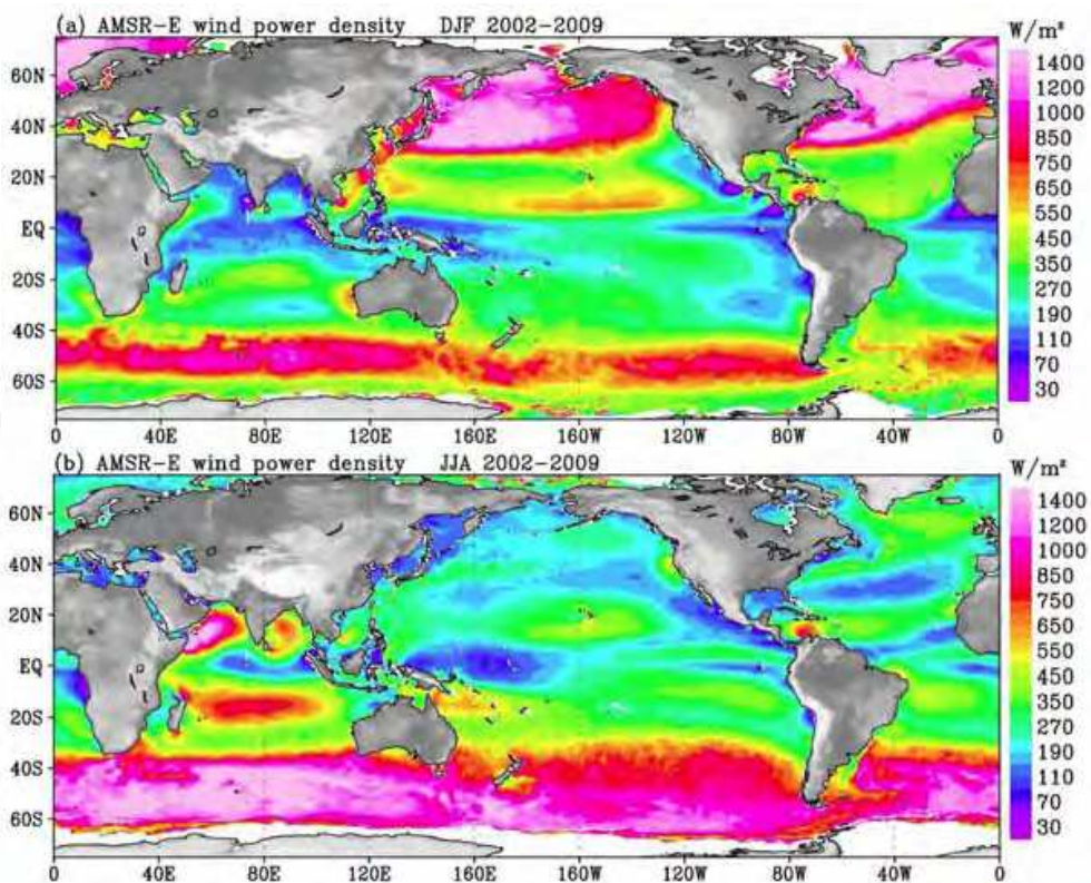
Fig. 3 Same as Fig. 2, but from AMSR-E.
