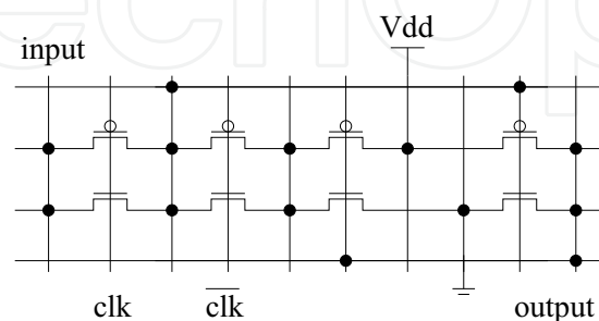
Fig. 7. An RDG-CNFET based latch implementation.
