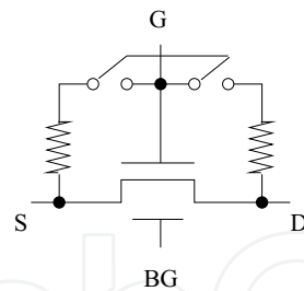
Fig. 4. Compact model of a n-type MOSFET-like reconfigurable double gate carbon nanotube field effect transistor (RDG-CNFET).
