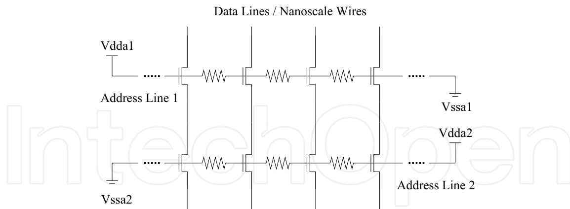
Fig. 8. Schematic of the proposed voltage-controlled nano-addressing circuit.
