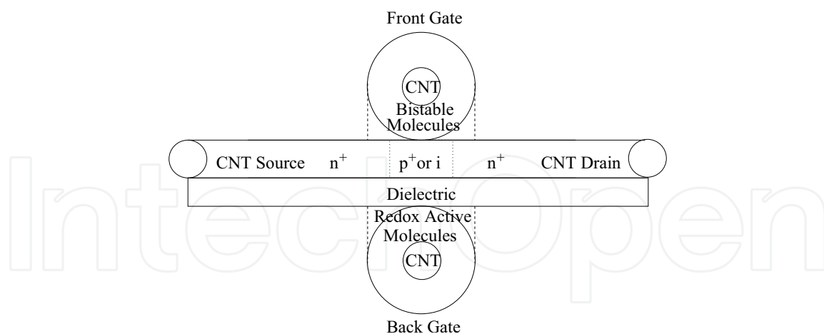
Fig. 3. A n-type MOSFET-like reconfigurable double gate carbon nanotube field effect transistor (RDG-CNFET).
