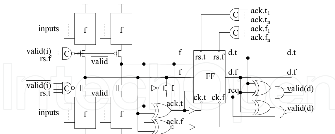
Fig. 11. A static logic based RDA (robust differential asynchronous) circuit.
