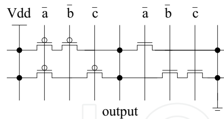
Fig. 6. An RDG-CNFET based Boolean logic a(b+c) implementation.
