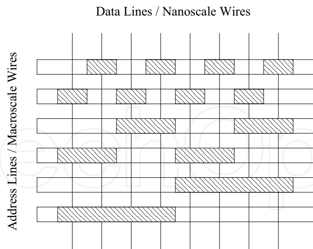
Fig. 2. Layout of undifferentiated nanoscale wires (data lines) addressed by microscale wires (address lines). Lithography defines high- and low-k dielectric regions, which gives field effect transistors and direct conduction, respectively.
