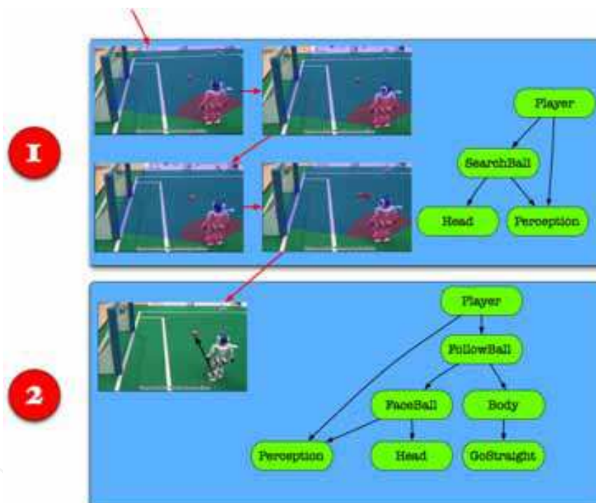
Fig. 29. Ball searching sequence.
