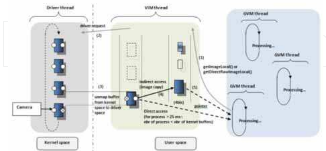
Fig. 5. Access to an image in the NaoQi framework.
