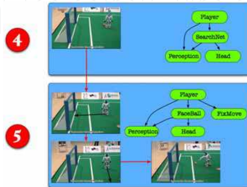
Fig. 31. Search net behavior and kick.
