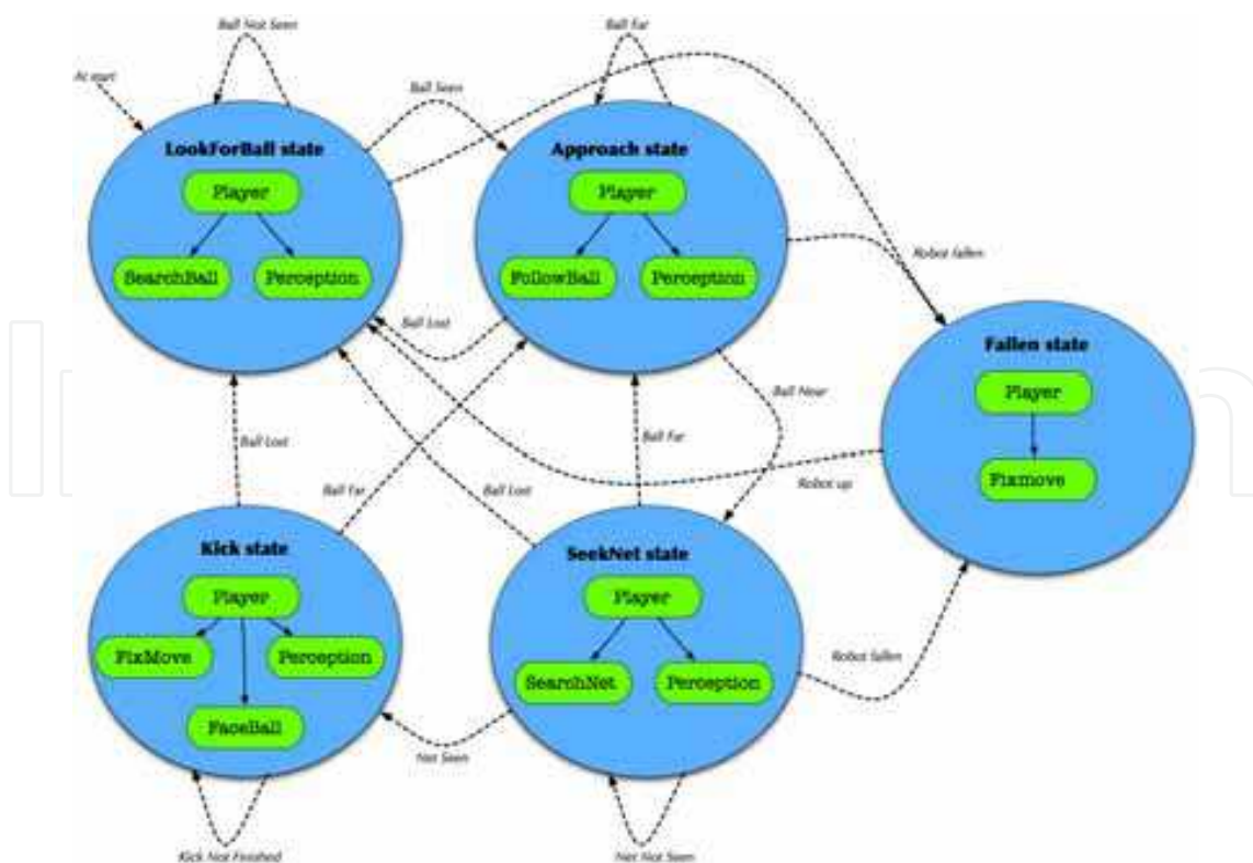
Fig. 25. Player component finite state machine with its corresponding activation tree.
