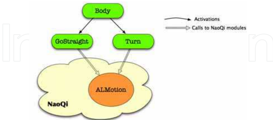
Fig. 21. Body component and its lower level components, which communicate with NaoQi to move the robot.
