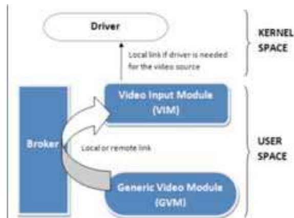
Fig. 4. NaoQi vision architecture overview.
