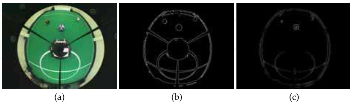
Fig. 10. Example of a captured image using the proposed approach. The cross over the ball points out the detected position. In b) the image a), with the Canny edge detector applied. In c), the image b) after applying the circular Hough transform.
