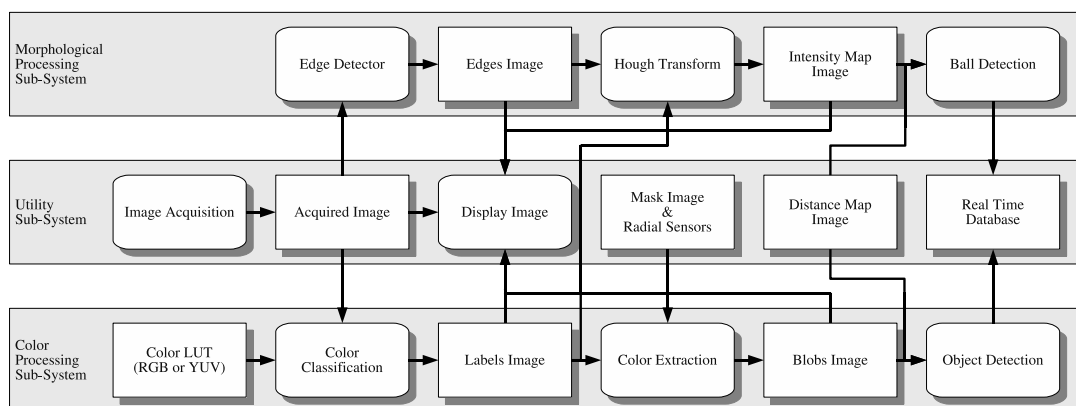
Fig. 4. The software architecture of the vision system developed for the CAMBADA robotic soccer team.
