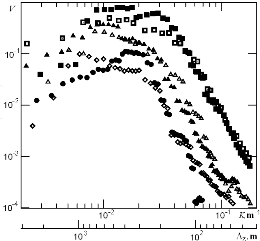
Fig. 4.7.9 Examples of the experimental spectrum v_n(K_y) as function of vertical wave number.
