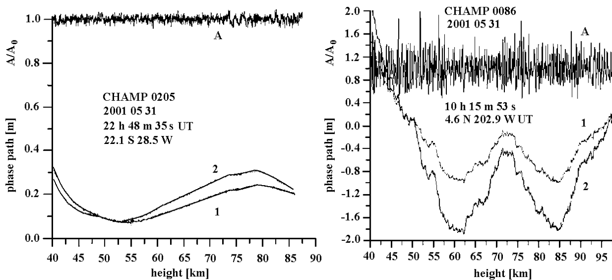
Fig. 5.1.1. Left panel. Quiet ionospheric conditions ( \text{rms}=0.0136 ), CHAMP RO event No. 0205, May, 31, 2001. Insert indicates the date, time of event, and coordinates of the ray perigee. Right panel. Noisy CHAMP event with high amplitude variations ( \text{RMS}=0.2191 ) in the equatorial region at the local midnight.
