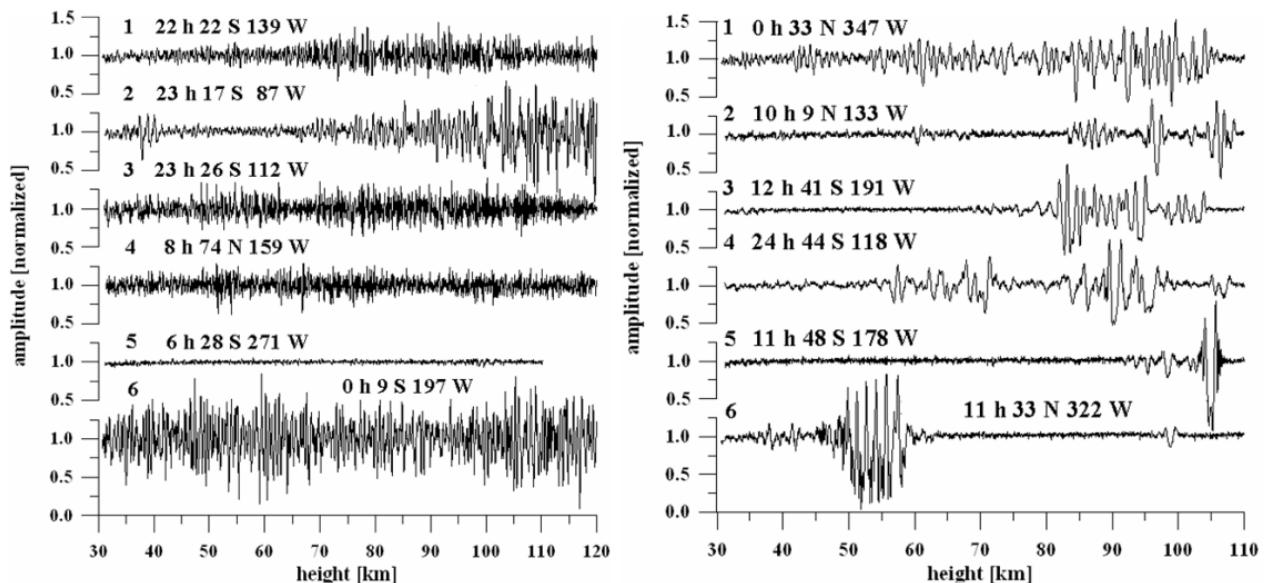
Fig. 5.3.1. Left panel: C-type noisy amplitude scintillations of RO signal. Right panel: S-type quasi-regular amplitude variation. Legends indicate the local time (LT) and the geographical coordinates of RO measurements
