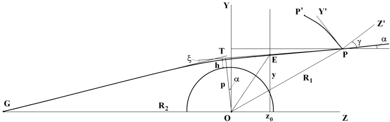
Fig. 3.3.1. Geometrical parameters for GIO, RFSA, CT and BP methods.
