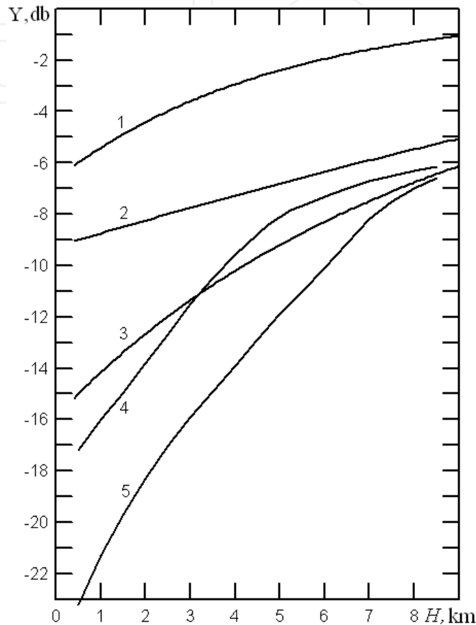
Fig.6.2.10. Different components of the attenuation of radio wave at wavelength \lambda = 2 cm.
