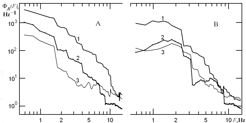
Fig. 4.7.13. The typical spectra of the amplitude fluctuations \Phi_a(F) of the decimeter radio waves.
