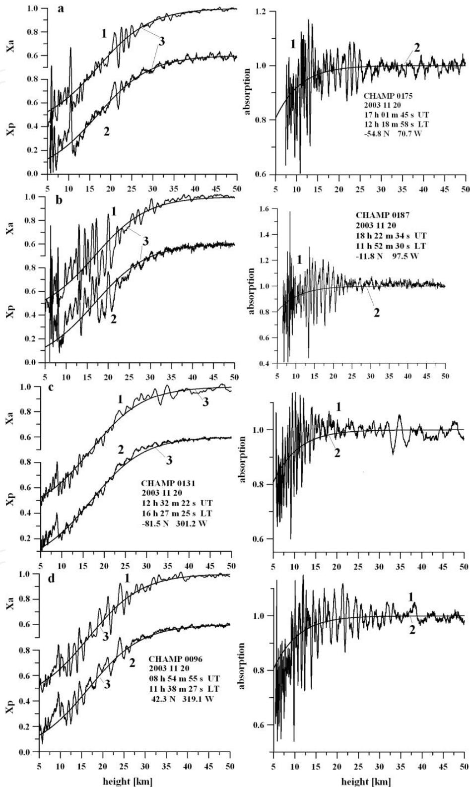
Fig. 4.6.2. The refractive attenuation and total absorption of radio waves in the atmosphere.
