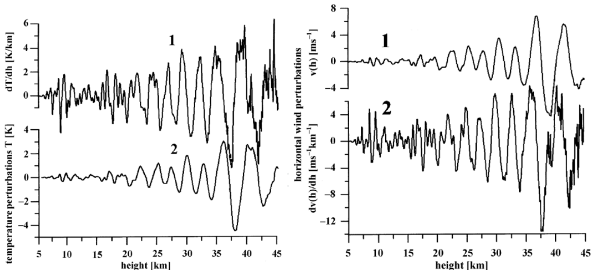
Fig. 4.5.4. Vertical profiles of the restored temperature variations and its gradients (left). Vertical profiles of the perturbation wind velocity (1) and its gradients (2) (right).
