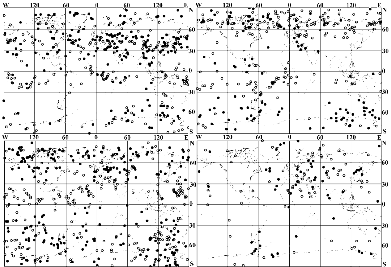
Fig. 5.5.2. Seasonal dependence of the global distribution of CHAMP RO events with intense amplitude variations (with magnitude of S_4 index greater than 0.2) for periods May 14–July 14, 2001, (left top panel), November–December 2001 (right top panel), October 28–November 26, 2003 (left bottom panel), July 2004 (right bottom panel). The day time events are marked by closed circles (local time 08–20 hours), the night-time events are indicated by open circles (local time 20–08 hours).
