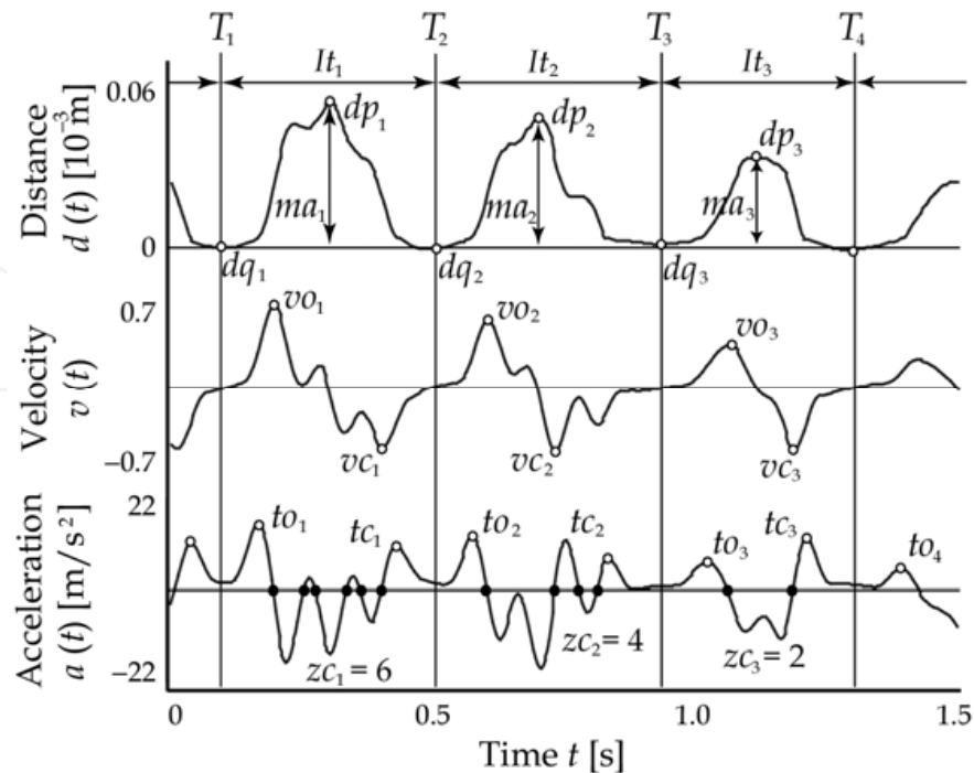
Fig. 3. Examples of the signals measured
