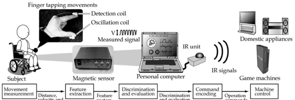
Fig. 1. Overview of the evaluation and training system for finger tapping movements
