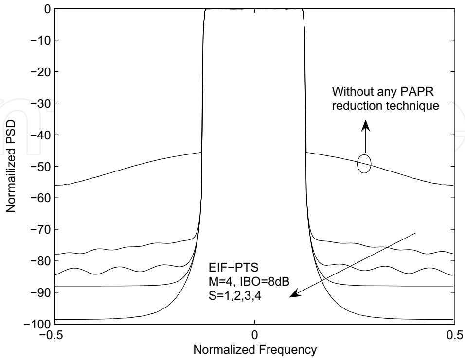
Fig. 8. Power Spectral Density of the EIT-PTS technique, when IBO = 8dB , M = 4
