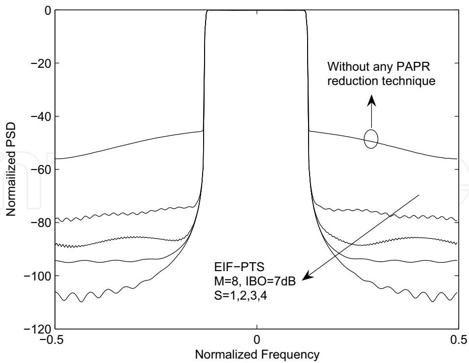
Fig. 9. Power Spectral Density of the EIT-PTS technique, when IBO = 7dB , M = 8
