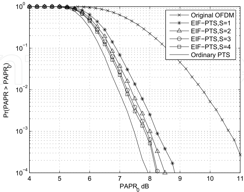
Fig. 3. Performance of EIF-PTS, M = 4
