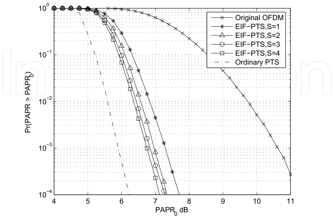
Fig. 5. Performance of EIF-PTS, M = 8
