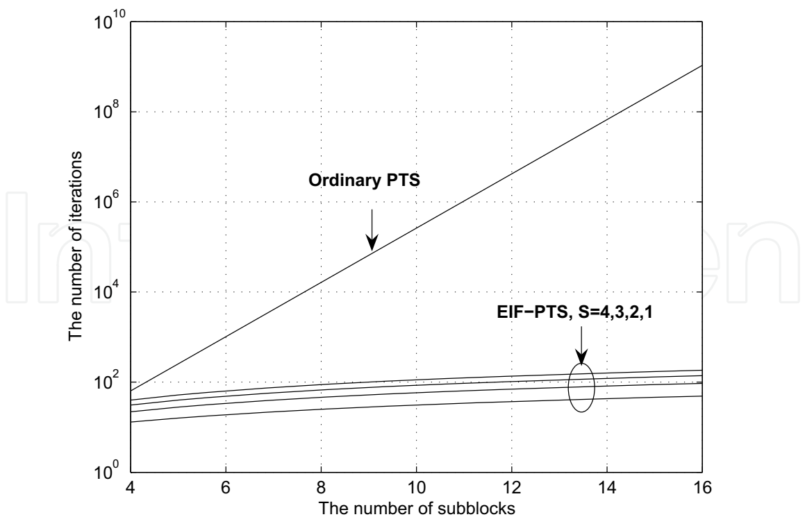
Fig. 6. Comparison of complexities between ordinary PTS and proposed EIF-PTS, W = 4
