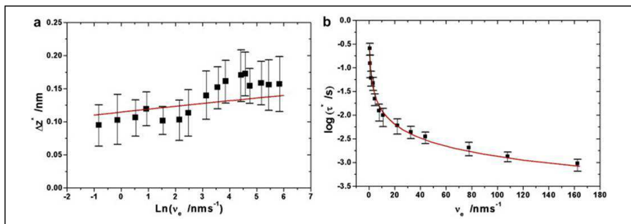
Fig. 9. Dynamic rupture of a \text{Au}_4 nanowire: a) Breaking distance as a function of the logarithm of the elongation rate v_e . The full line shows the calculations according to the present model and the squares are data for gold point contacts taken from (Huang et al., 2007a). The segments show the width of the distribution reported there. No fitting parameters were considered. b) Logarithm of the lifetime of the wire, \tau^* , as a function of the decimal logarithm of the elongation rate, v_e . The full line shows the calculations according to the present model and the squares are experimental data for the rupture of the Au - ODT taken from (Huang et al., 2007a). The segments show the width of the distribution reported there. No fitting parameters were considered. Reprinted from Vélez, P.; Dassie, S. A.; Leiva, E. P. M. Chem. Phys. Lett. , Vol. 460, No.1-3, 261-265, 2008 with permission from Elsevier.
