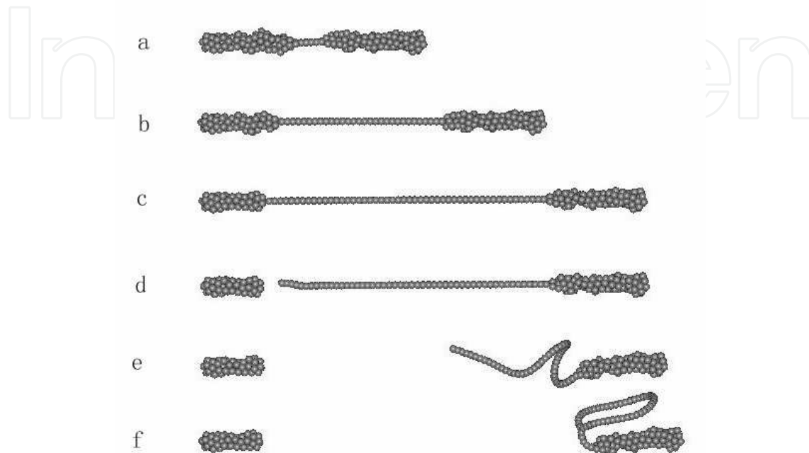
Fig. 5. Three-dimensional views of morphological changes (axial deformation) for CNW (A2) (a) At \epsilon=0.25 the middle part forms a single chain. (b) At \epsilon=1.0 the atomic chain stretches further. (c) At \epsilon=1.62 the CNW has stretched to the maximum. (d) At \epsilon=1.63 the atomic chain breaks. (e) The broken end recoils. (f) The broken end recoils, meeting with the single chain to form a loop.
