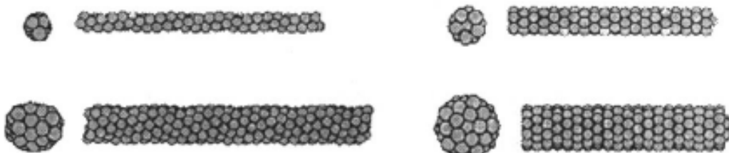
Fig. 16. Morphologies of structural growth sequences in selected nickel nanowires. The nanowire from the top to bottom on the left-hand side corresponds to W3-1, W3-2, and the nanowire from the top to bottom on the right-hand side corresponds to W5-1, W5-2, respectively.
