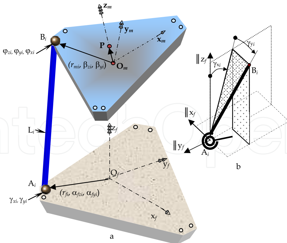
Fig. 2. The structure of the Stewart-DELTALAB platform (a) and of the leg i (b)
