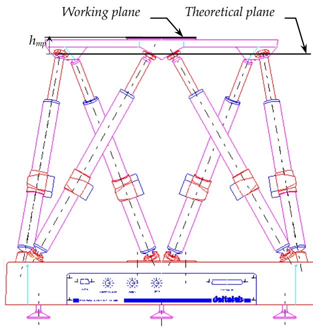
Fig. 6. Theoretical and working planes of Stewart platform
