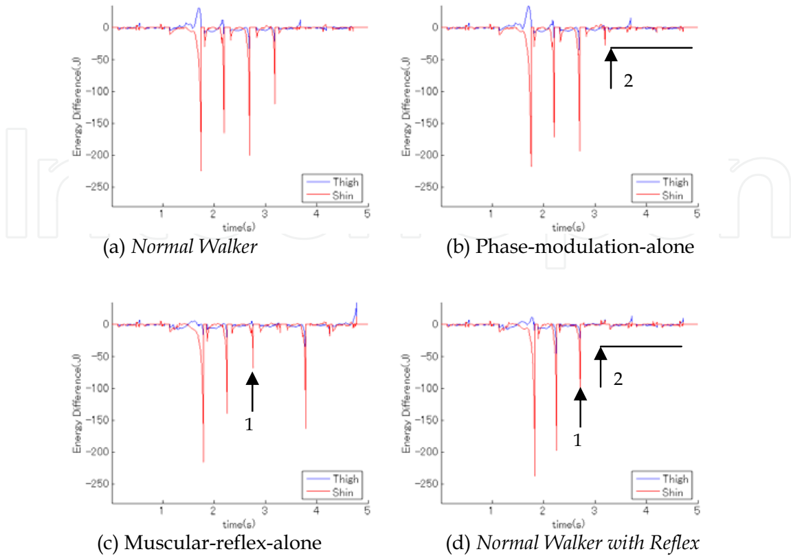
Fig. 8. Energy Difference
