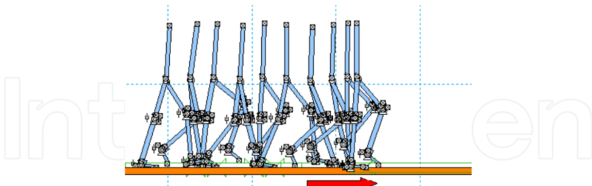
Fig. 13. Stick graph of the Spastic Walker with Reflex (the arrow denote the slip period): the Spastic Walker with Reflex kept its balance after slip perturbation.
