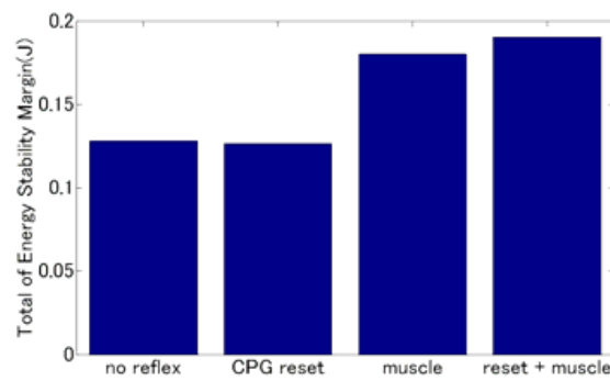
Fig. 7. Integration of Energy Stability Margin (from left, Normal Walker, Normal Walker with phase modulation, Normal Walker with muscular reflex, Normal Walker with Reflex)
