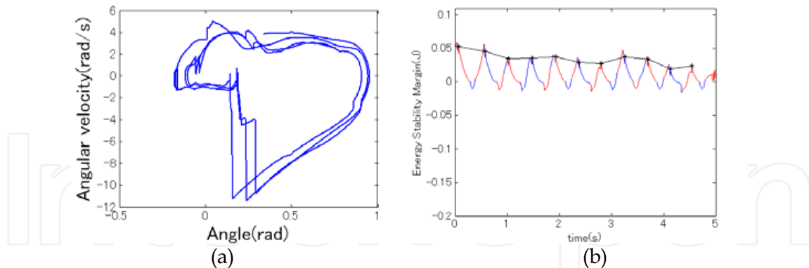
Fig. 12. (a) Phase portrait of the hip joint angle: and (b) Five seconds of the Energy Stability Margin of Spastic Walker
