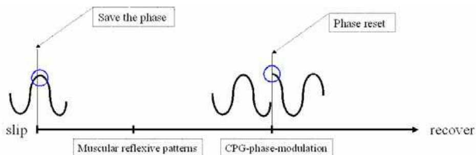
Fig. 4. CPG-phase-modulation
