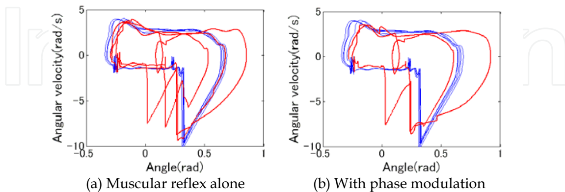
Fig. 10. Phase portraits of the hip joint angle ( Normal Walker )
