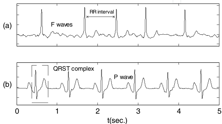
Fig. 1. Comparison between Atrial Fibrillation (a) and Normal Sinus Rhythm (b)
