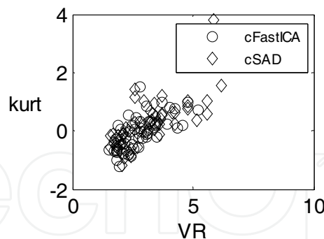
Fig. 8. Scatter plot between VR and kurtosis values
