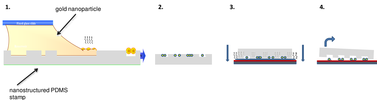
Scheme 2. Generation of 100nm gold nanoparticles arrays by directed assembly. 1) Capillary assembly of gold nanoparticles on a nanostructured PDMS stamp. 2) Nanostructured PDMS stamp with assembled gold nanoparticles. 3) The assembly is then transfer-printed with solvent mediation. 4) The PDMS stamp is finally peeled away.
