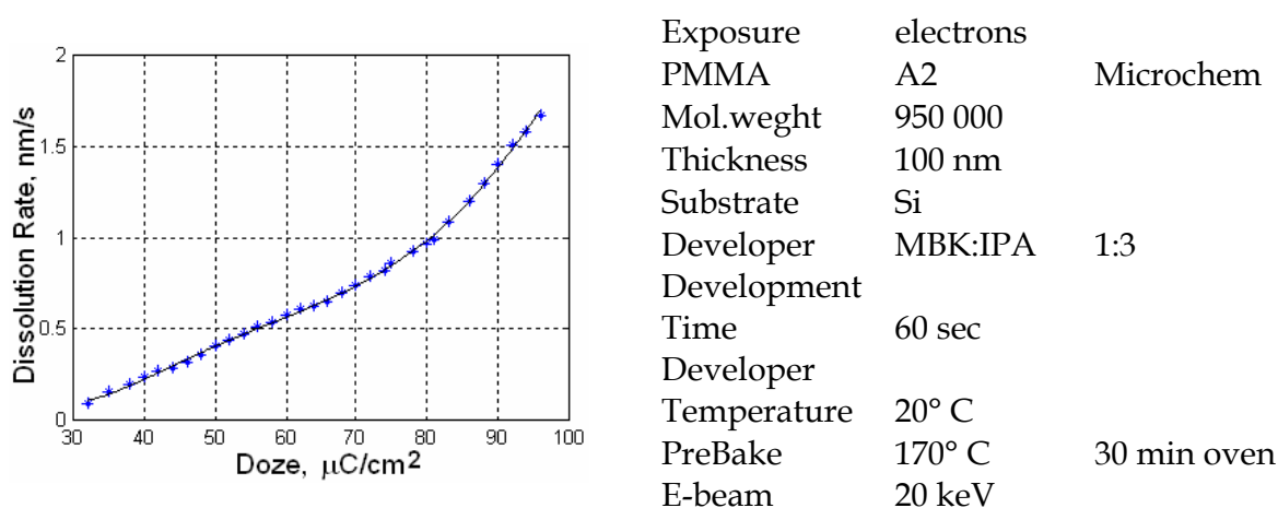
Fig. 5. Dissolution rate, calculated for PMMA at the given parameters (100nm, 20keV)
