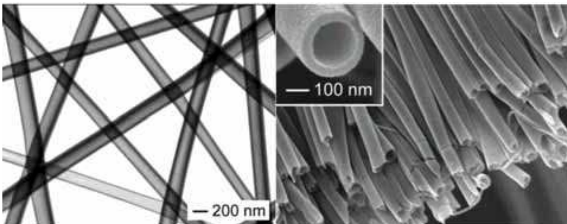
Fig. 3. TEM image (left) and SEM image (right) of \text{TiO}_2/\text{PVP} hollow fibers fabricated by coaxial electrospinning.
