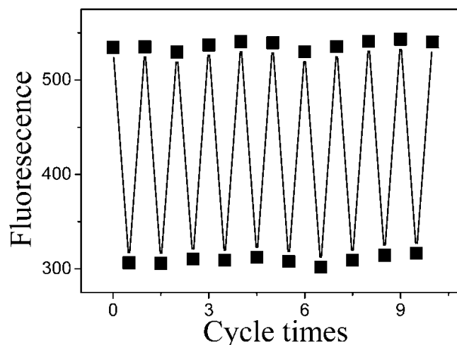
Fig. 17. The thermochromic cycle reversibility experiment of CBT-PMMA nanofibers' film. In each cycle, the fluorescent emission at \lambda = 503 nm of the samples was monitored at 10^\circ\text{C} and 50^\circ\text{C} , respectively.
