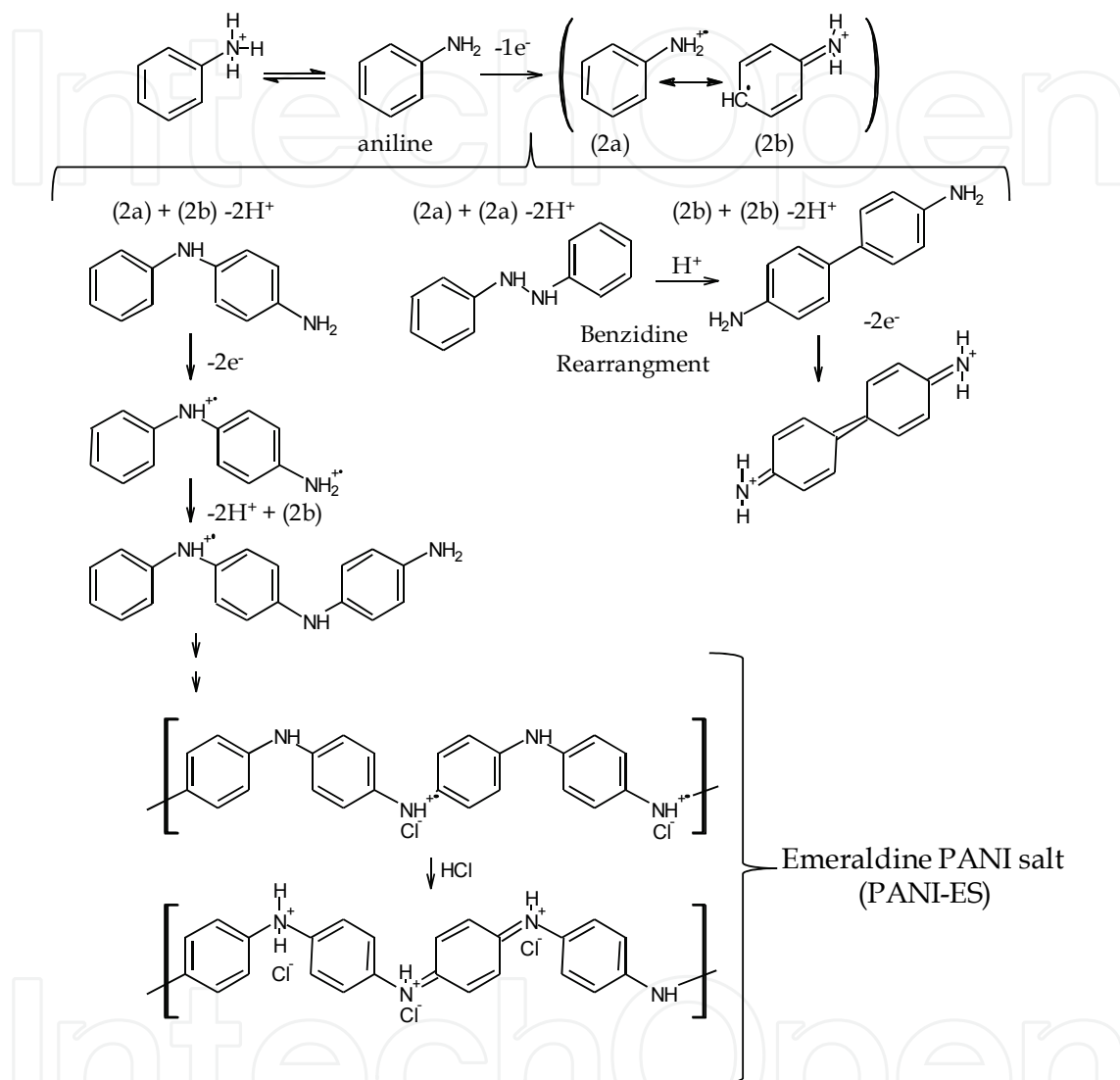
Fig. 3. Schematic representation of the polymerization steps present during the aniline polymerization. The structure of PANI is shown with radical cations (or polarons) and dications (bipolarons) segments.
