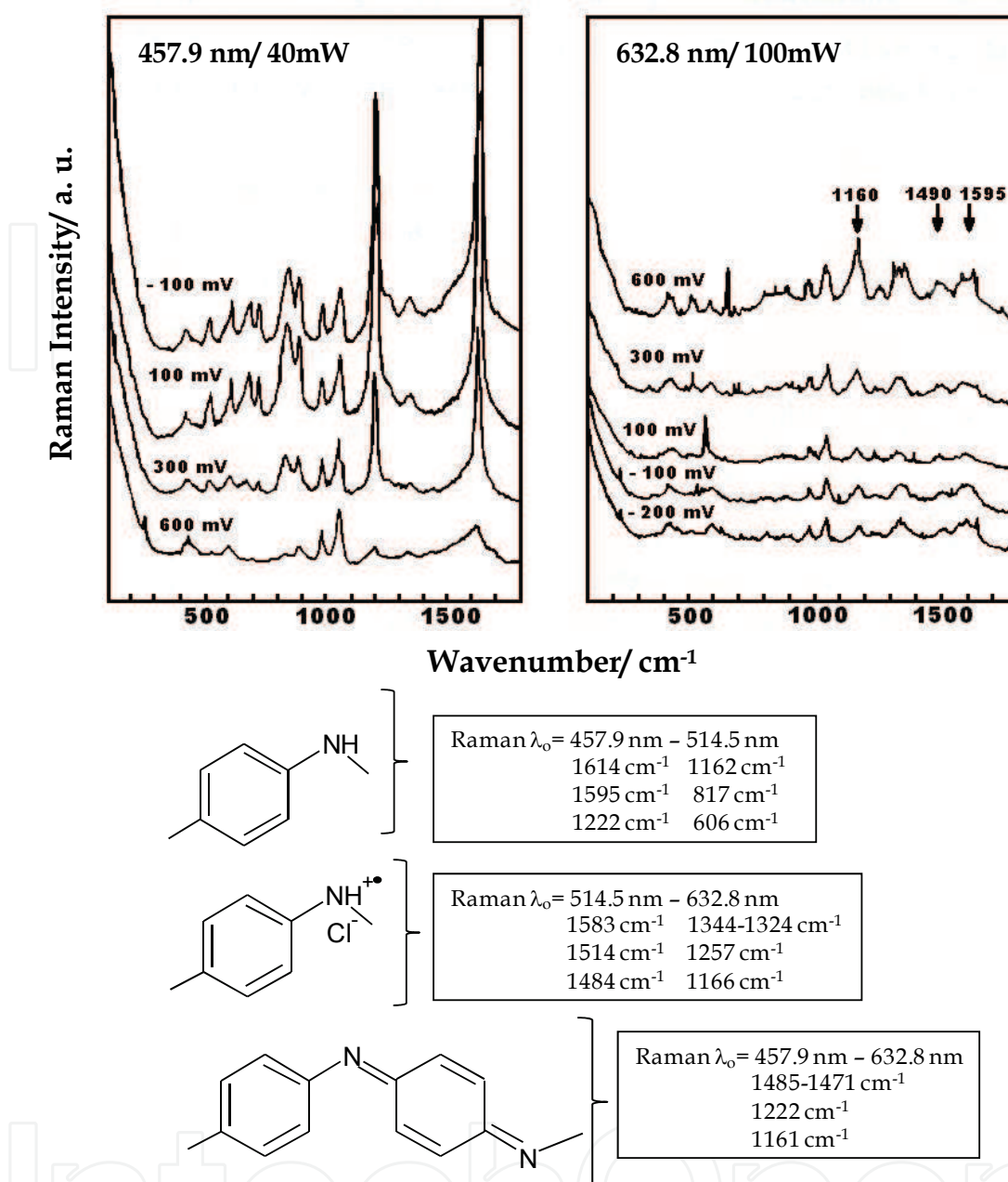
Fig. 6. Top: Raman spectra of PANI in different oxidation stages (the applied voltage is indicated in the figure) at indicated laser line (457.9 nm and 632.8 nm). Reproduction authorized by Elsevier (Sacricifti & Kusmany, 1987). Bellow: schematic representation of segments of PANI and its characteristic Raman bands at indicated laser lines (Furukawa et al., 1988).
