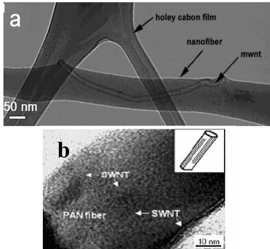
Fig. 3. a) TEM image of protrusion of MWNTs from the fibre [128] [Copyright ACS]. b) High resolution TEM image showing a uniform distribution and alignment of SWNTs in PAN fibre with the diameter of about 50nm [45] [Copyright Wiley-VCH].
