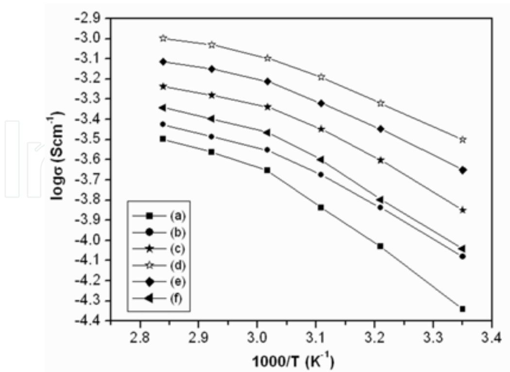
Fig. 16. \log \sigma vs. temperature inverse curve PEO-P(VdF-HFP)-LiClO 4 -x% dedoped polyaniline nanofibers polymer electrolyte membranes (a) x = 0, (b) x = 5, (c) x = 10, (d) x = 15, (e) x = 20 and (f) x = 25
