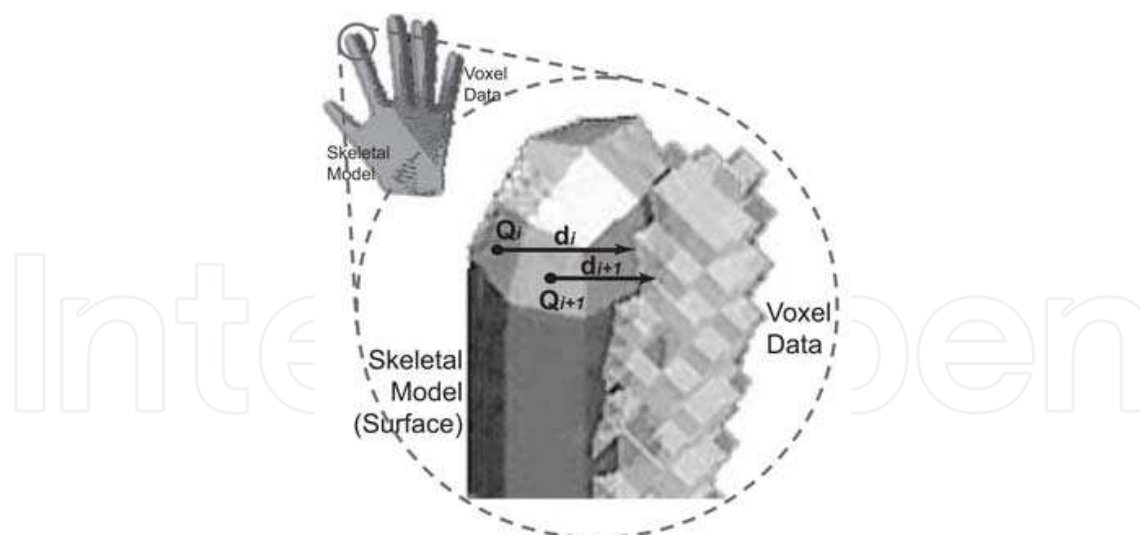
Fig. 5. The calculation of geometric error between surface model and voxel data.
